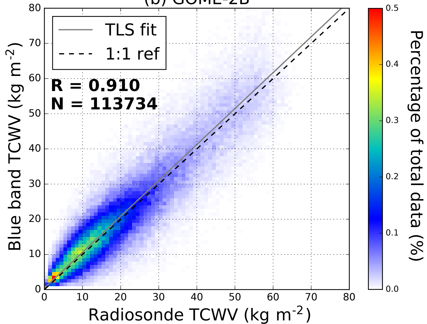
(b) GOME-2B
