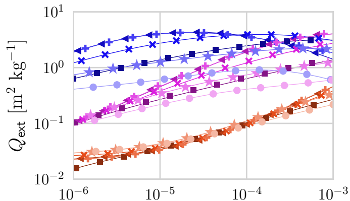
(b) 175.3 GHz
