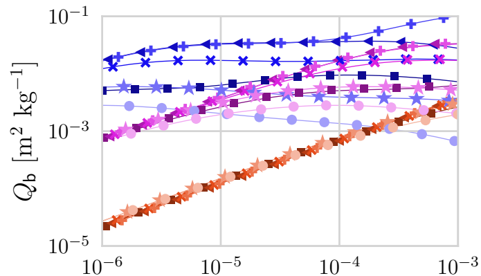
(a) 94.1 GHz
