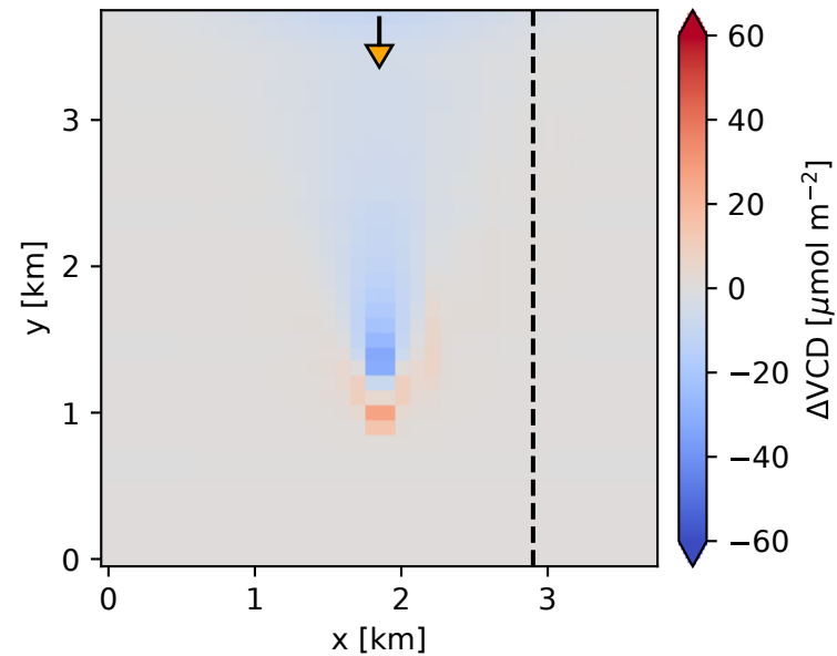
(c) \Delta VCD for SZA:40° and SAA:180°
