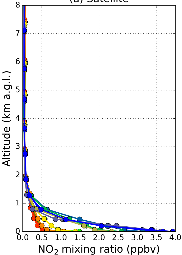
(a) Satellite
