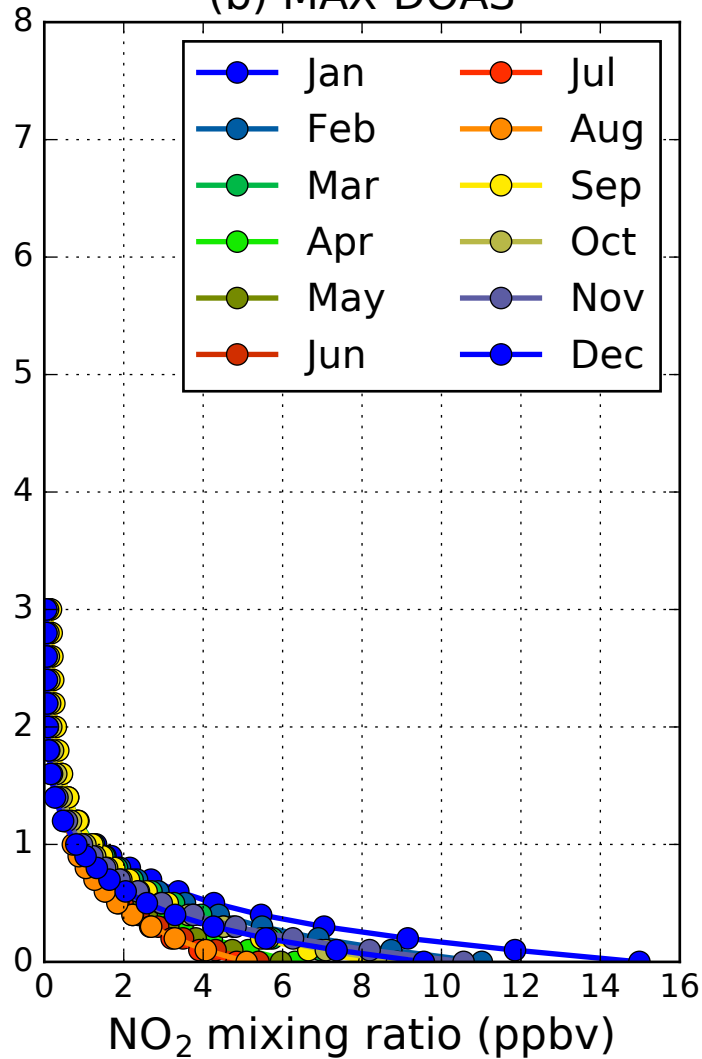
(b) MAX-DOAS
