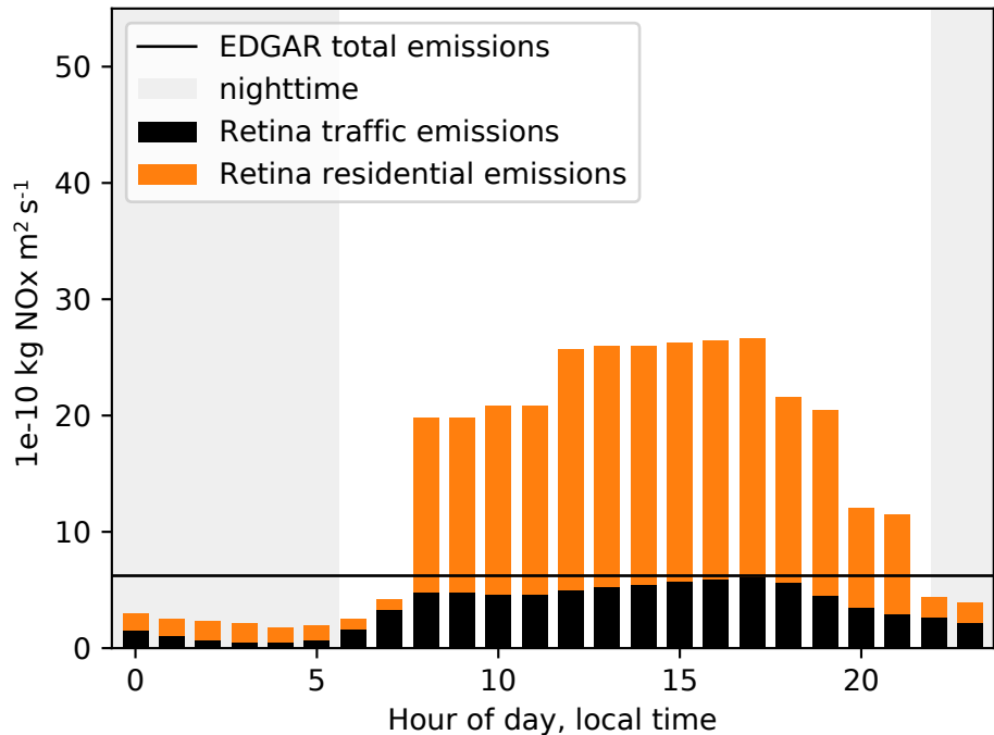
Amsterdam NOx emissions, summer (Jul 2016)
