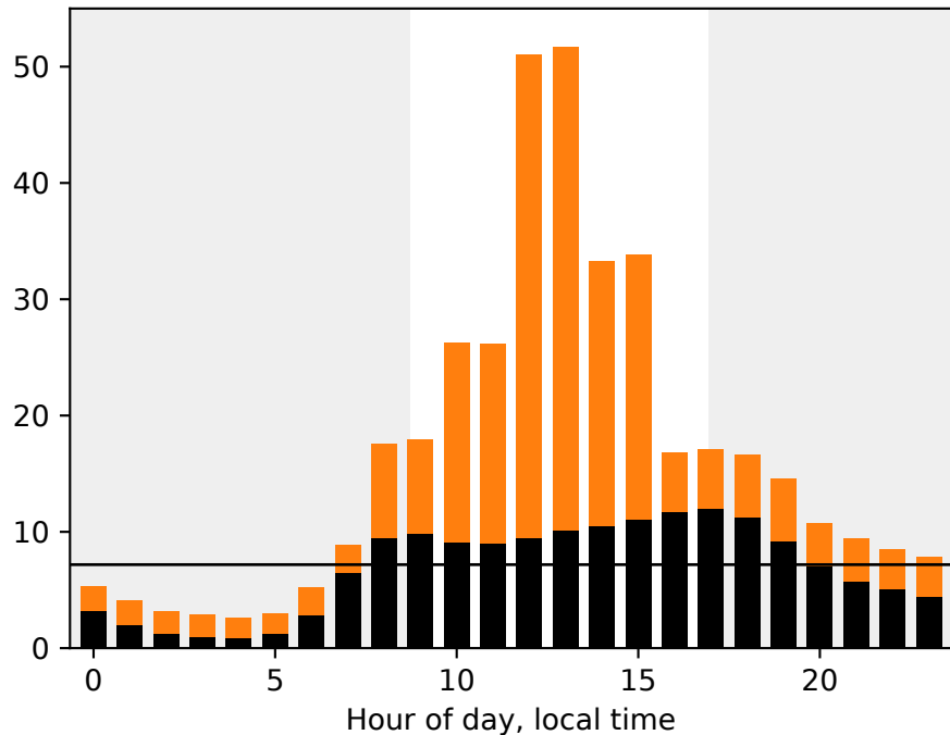
Amsterdam NOx emissions, winter (Jan 2017)
