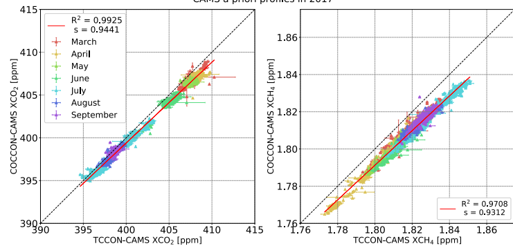
CAMS a priori profiles in 2017
