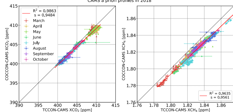
CAMS a priori profiles in 2018
