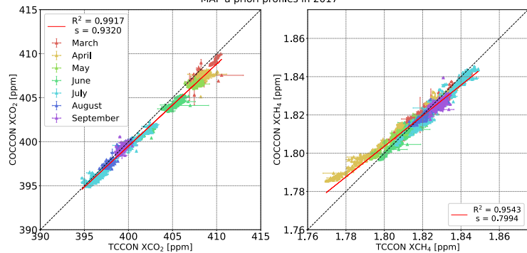
MAP a priori profiles in 2017
