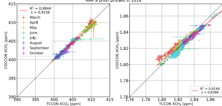
MAP a priori profiles in 2018
