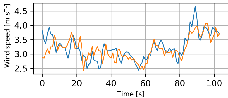
Height 18 m
