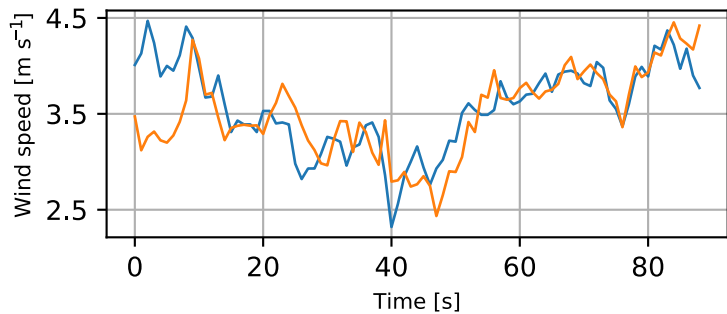
Height 31 m
