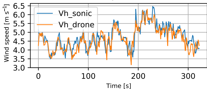
Height 57 m
