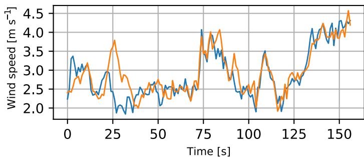
Height 18 m
