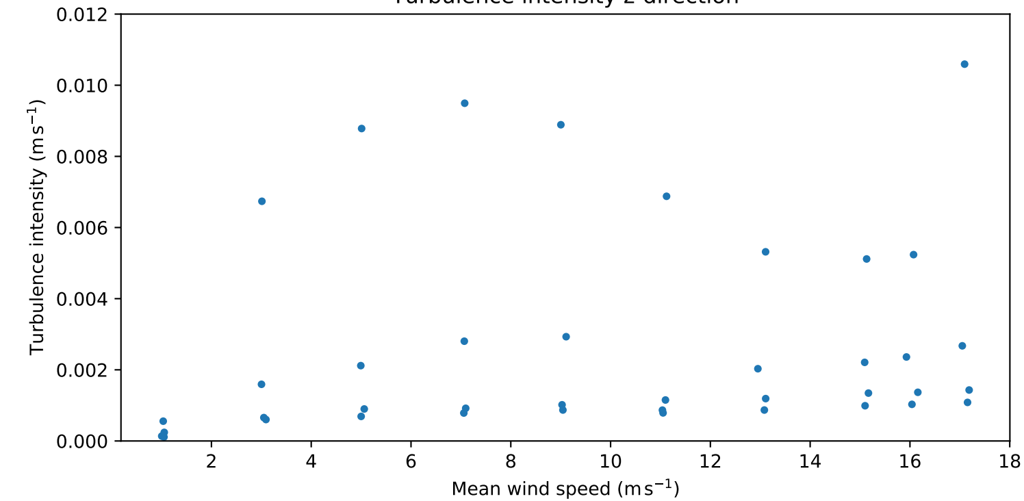
Turbulence intensity z direction
