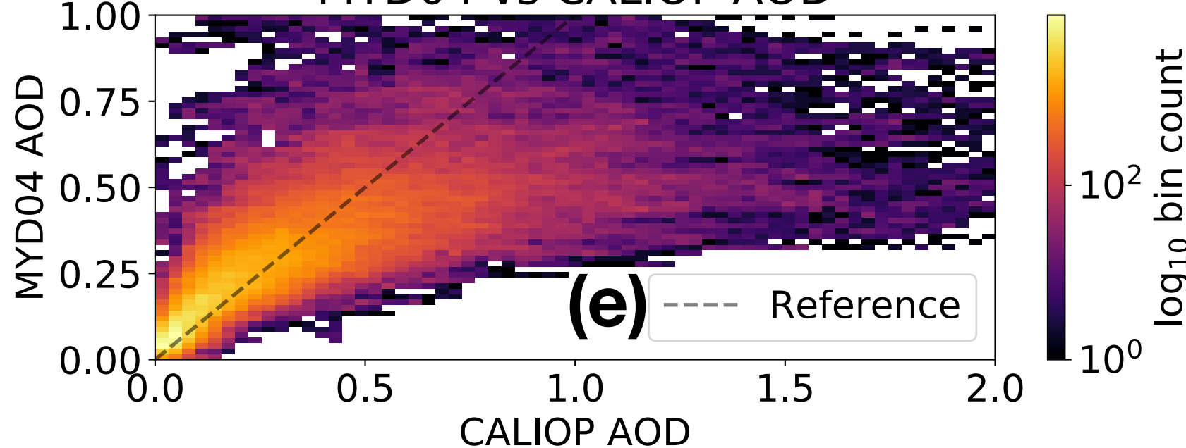
MYD04 vs CALIOP AOD
