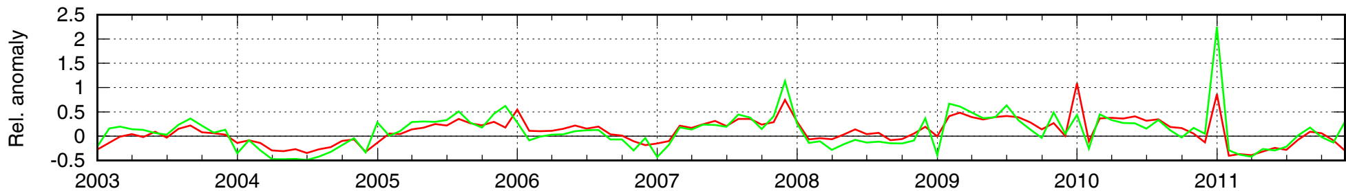
(c) Extinction at 25 km
