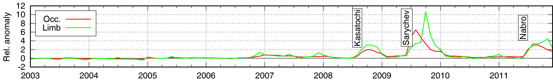
(a) Extinction at 15 km
