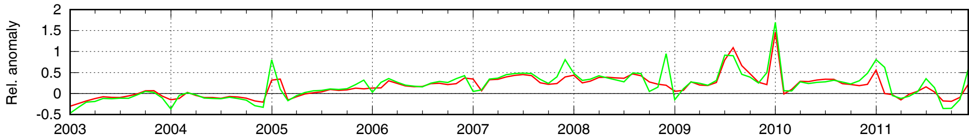
(b) Extinction at 20 km
