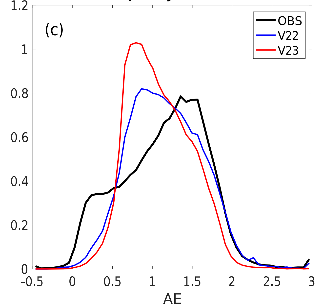
AE frequency distributions
