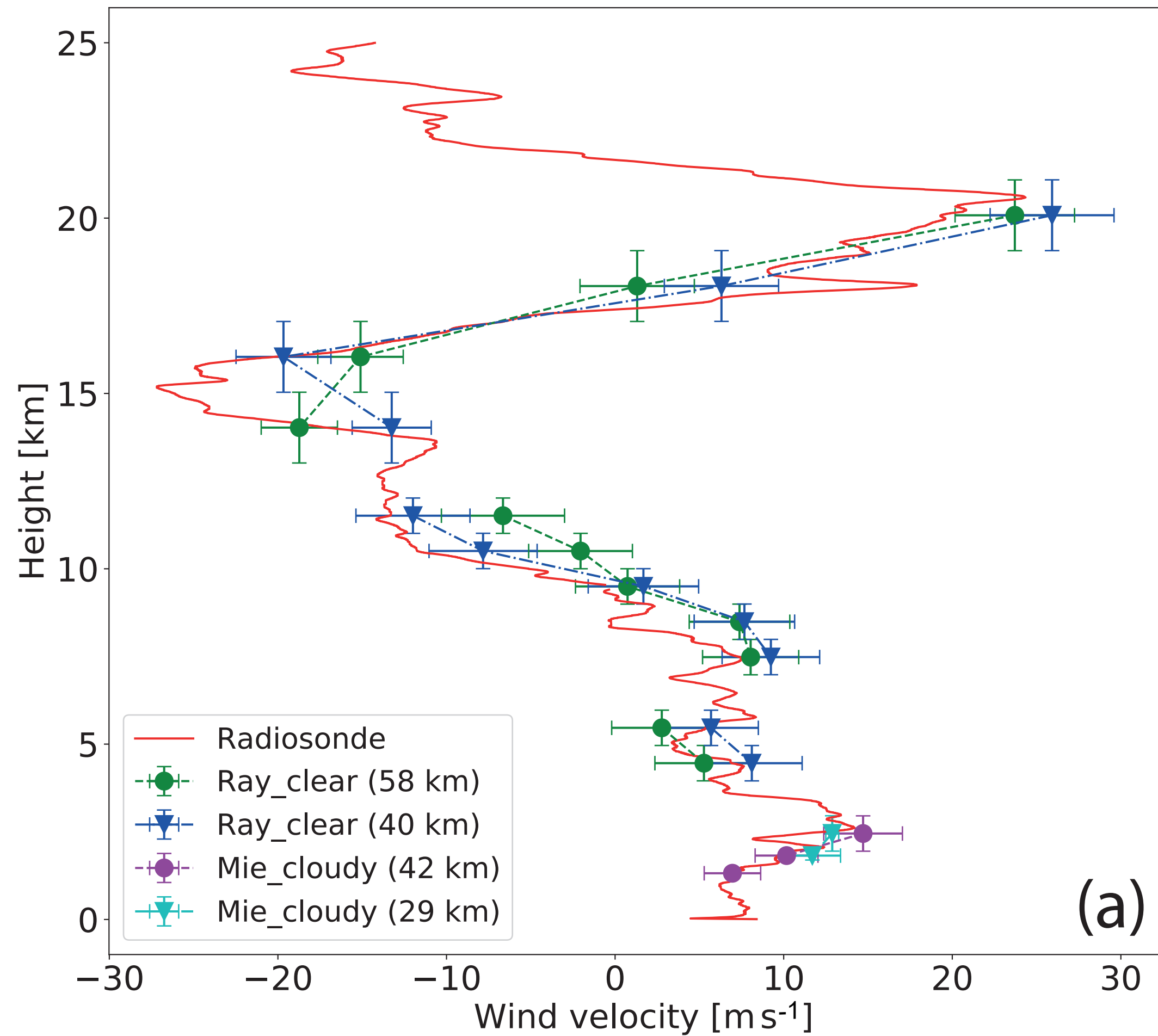
Radiosonde and Aeolus L2B wind
