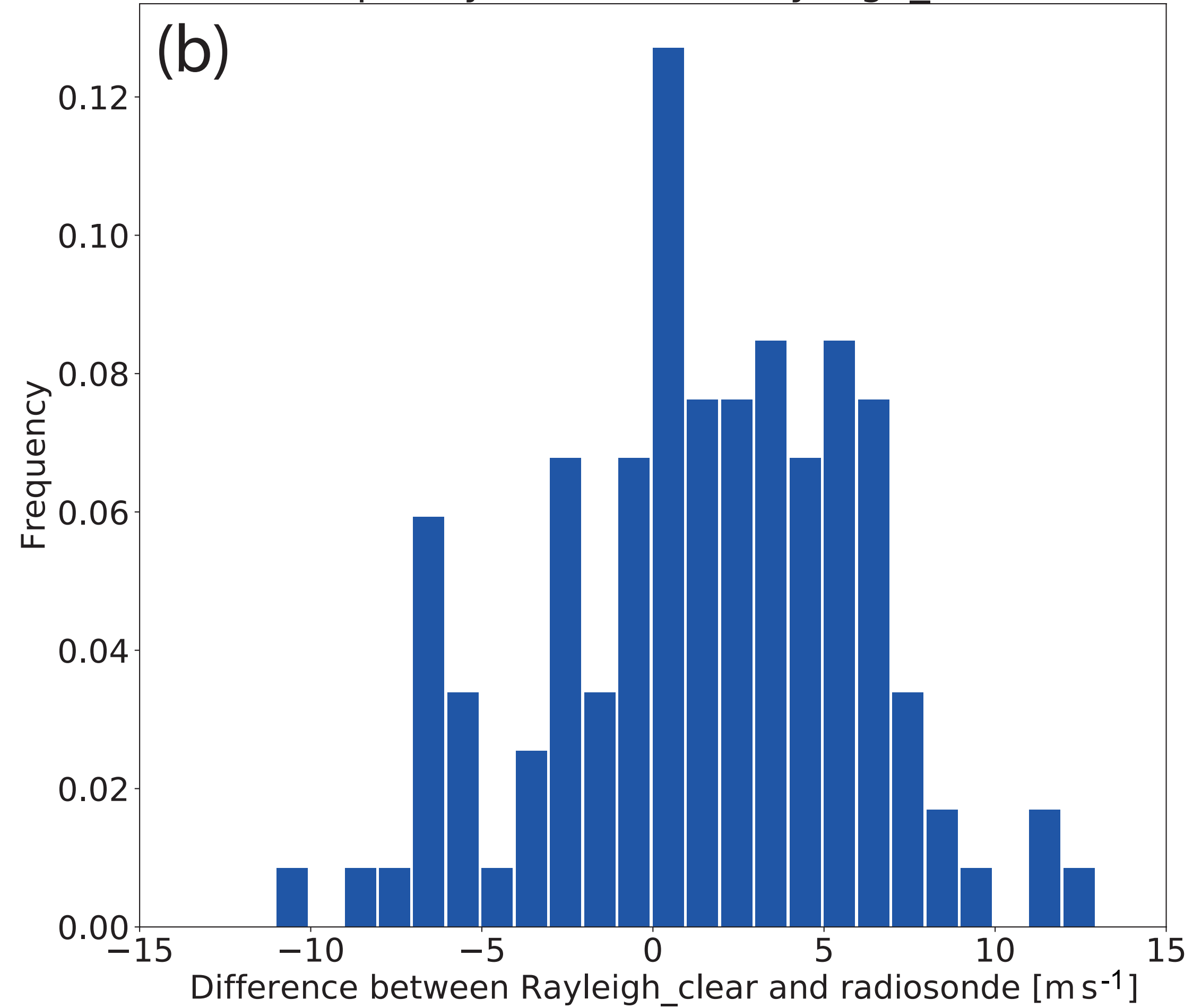
Frequency distribution Rayleigh_clear
