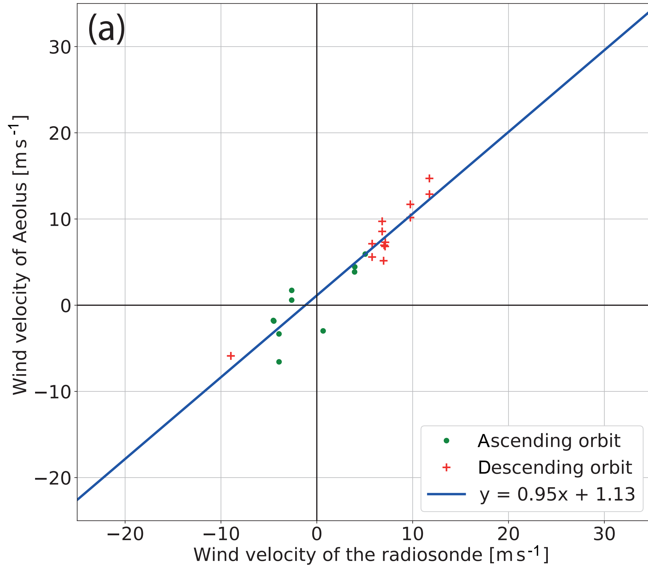
Mie L2B wind vs. radiosonde
