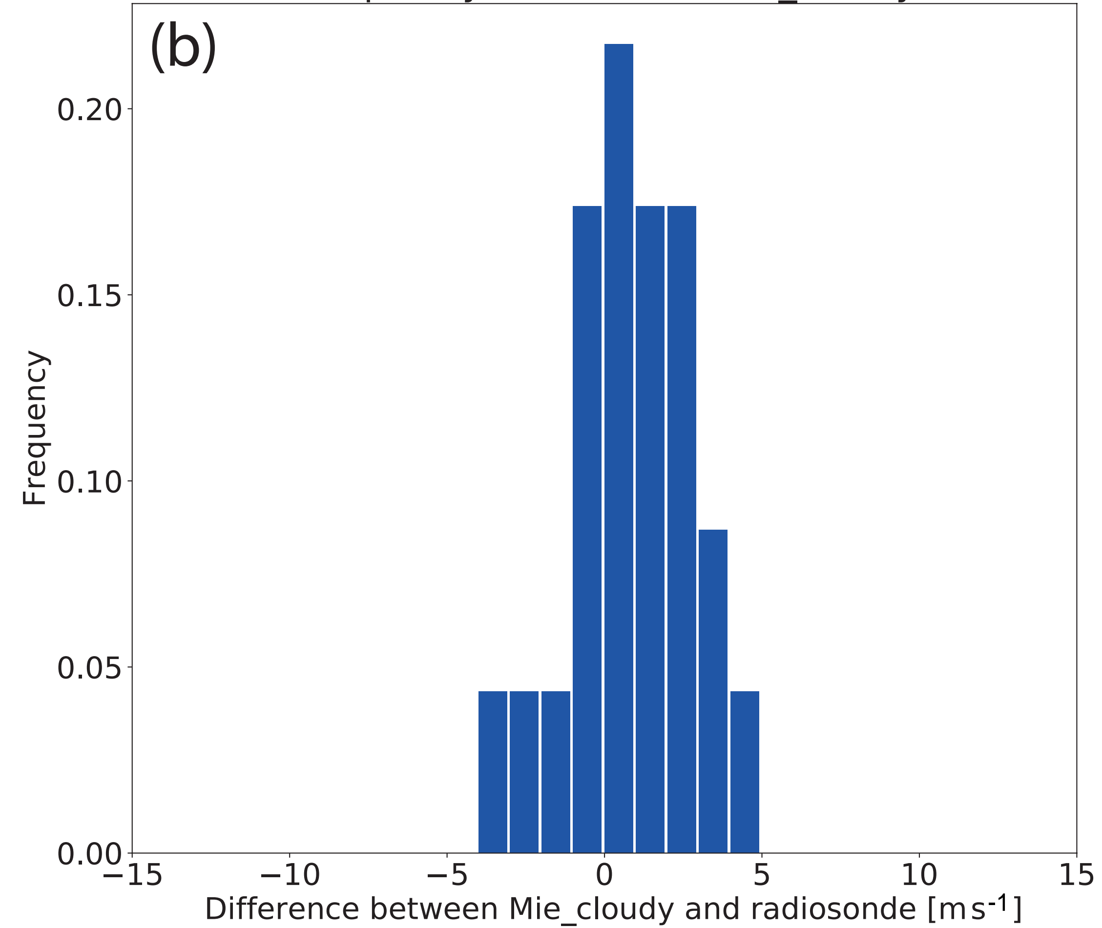
Frequency distribution Mie_cloudy
