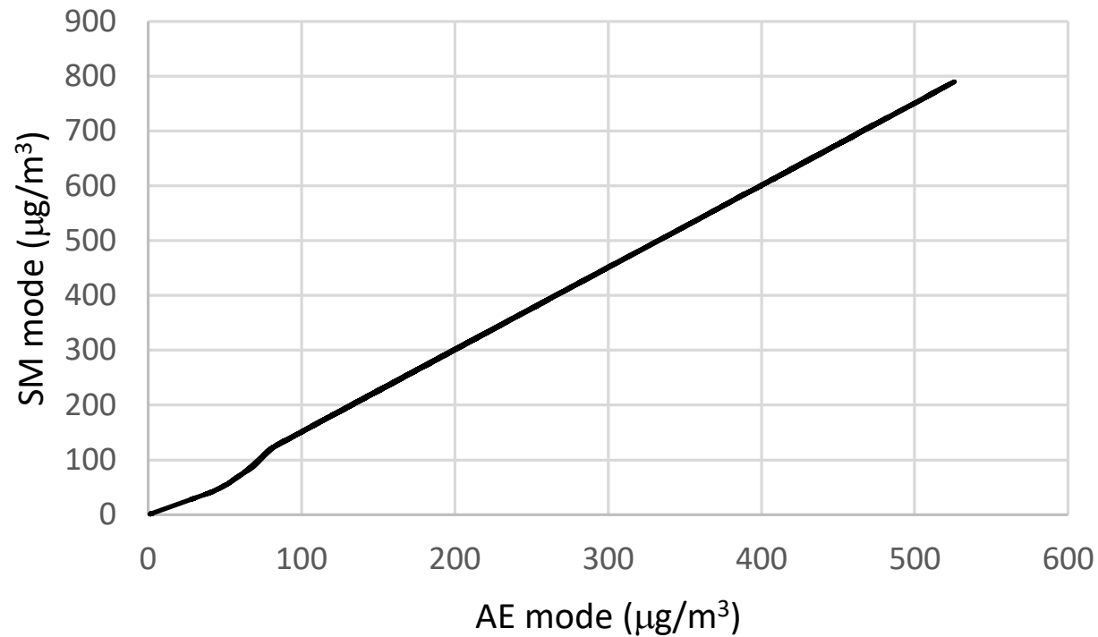
PMS5003, PM 10
