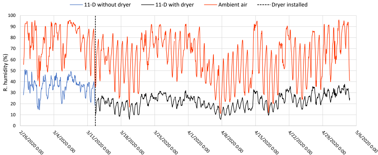
Diffusion dryer effect on Grimm 11-D, hourly average r. humidity
