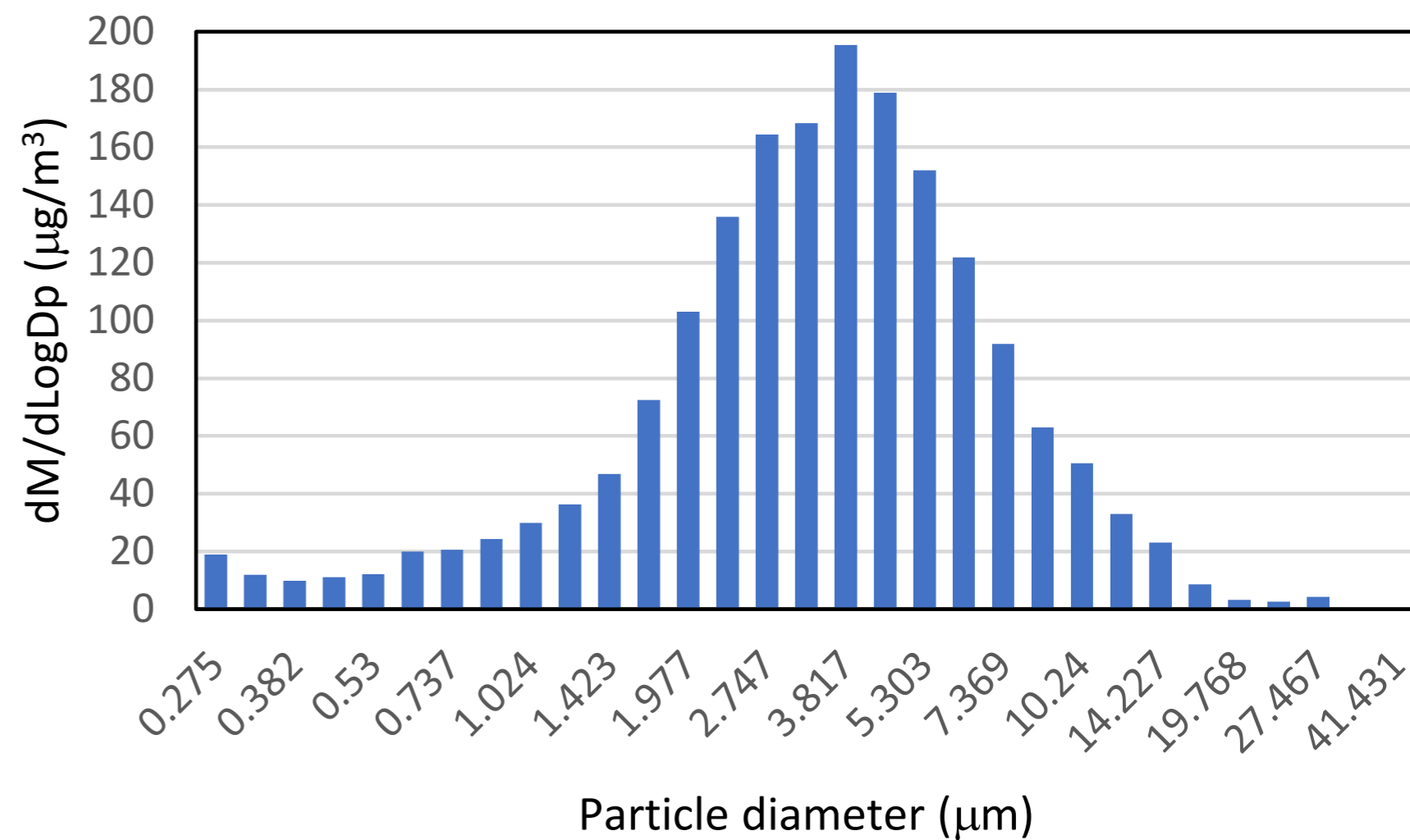
11-D mass distribution, 3/27/2020 20:00
