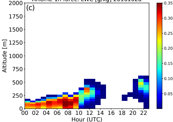
AROME 1h forec. LWC [g/kg] 20161028
