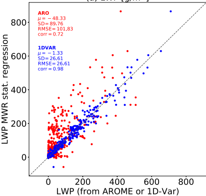
(a) LWP [ \text{g}/\text{m}^2 ]
