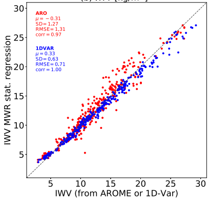
(b) IWV [ \text{kg}/\text{m}^2 ]
