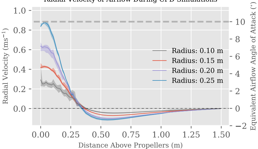
Radial Velocity of Airflow During CFD Simulations
