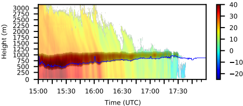
Attenuated equivalent reflectivity factor (dBZ)
