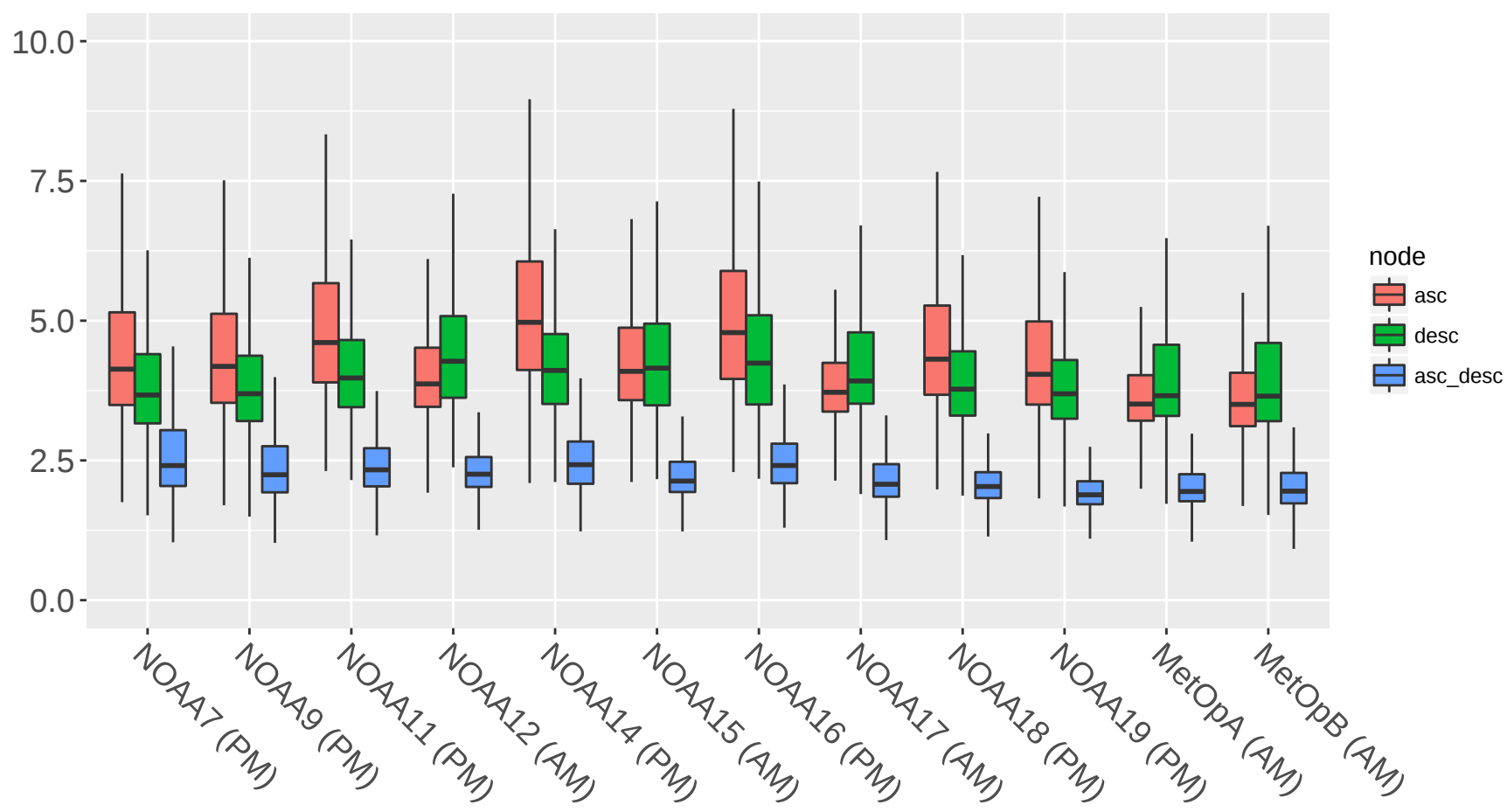
Bias-corrected RMSE (CFC[%])
