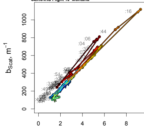
(b) Diagnosed MERET C_{\text{burn}} , ppm
