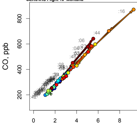
(a) Diagnosed MERET C_{\text{burn}} , ppm
