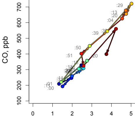
(c) Diagnosed MERET C_{\text{burn}} , ppm
