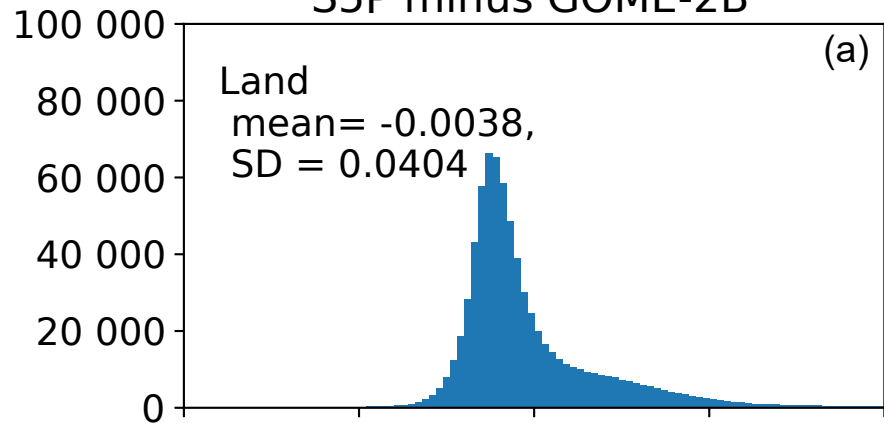
S5P minus GOME-2B
