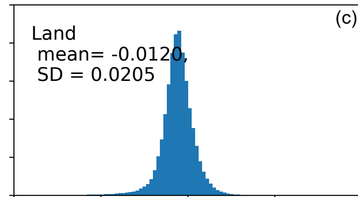
OMI minus GOME-2B
