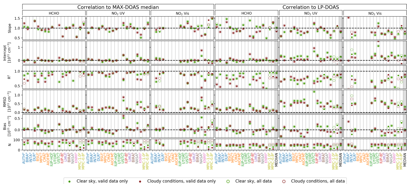
Figure S57. Correlation statistics of trace gas surface concentrations retrieved from the participant's own dSCDs. Basic description of Fig. S51 applies.
