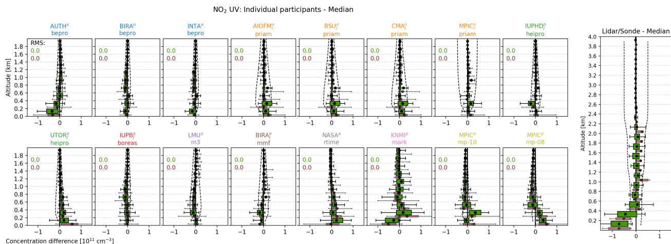
Figure S23. Deviations of NO 2 UV profiles (valid only) of individual participants from the MAX-DOAS median profiles. The description of Fig. S20 applies. On the right, deviation of the median retrieved profiles from the few available NO 2 lidar and sonde profiles are shown.
