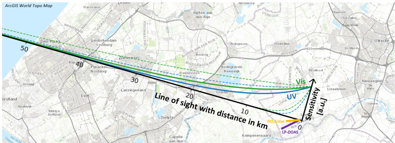
Figure S11. Line of sight of the MAX-DOAS instruments on a map (Esri et al., 2018). The coloured curves indicate the sensitivity for the average (solid), the minimum (dashed) and maximum (dashed) viewing distances encountered during the campaign in the UV (blue) and Vis (green).
