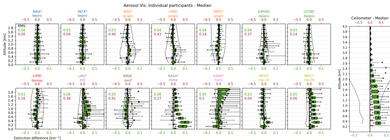
Figure S21. Deviations of Aerosol Vis profiles (valid only) of individual participants from the MAX-DOAS median profiles. Description of Fig. S20 applies.
