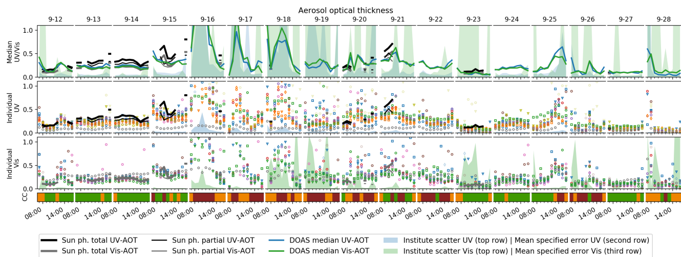
Figure S50. MAX-DOAS AOTs retrieved from the participant's own dSCDs in comparison to sun photometer data. Symbol and symbol colours are chosen according to Table 2 in the main text. Transparent symbols indicate data flagged as invalid. Top row: MAX-DOAS median results vs. the available supporting observations, according to the legend below the plot. The "institute scatter" areas show the scattering among the participants in terms of standard deviation with valid data considered only. Two lower rows: Comparison of the individual participants for the two spectral retrieval ranges. Here the coloured area is the average retrieval error, as specified by the participants.
