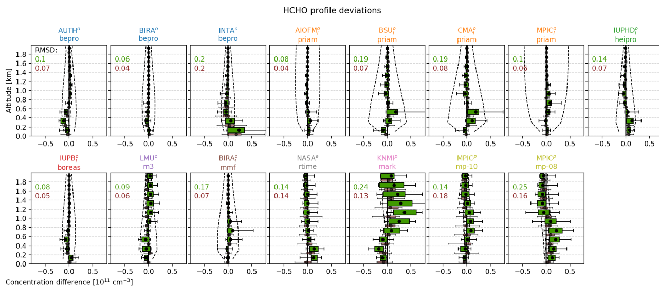
Figure S22. Deviations of HCHO profiles (valid only) of individual participants from the MAX-DOAS median profiles. The description of Fig. S20 applies but for HCHO, there is no independent reference profile available.
