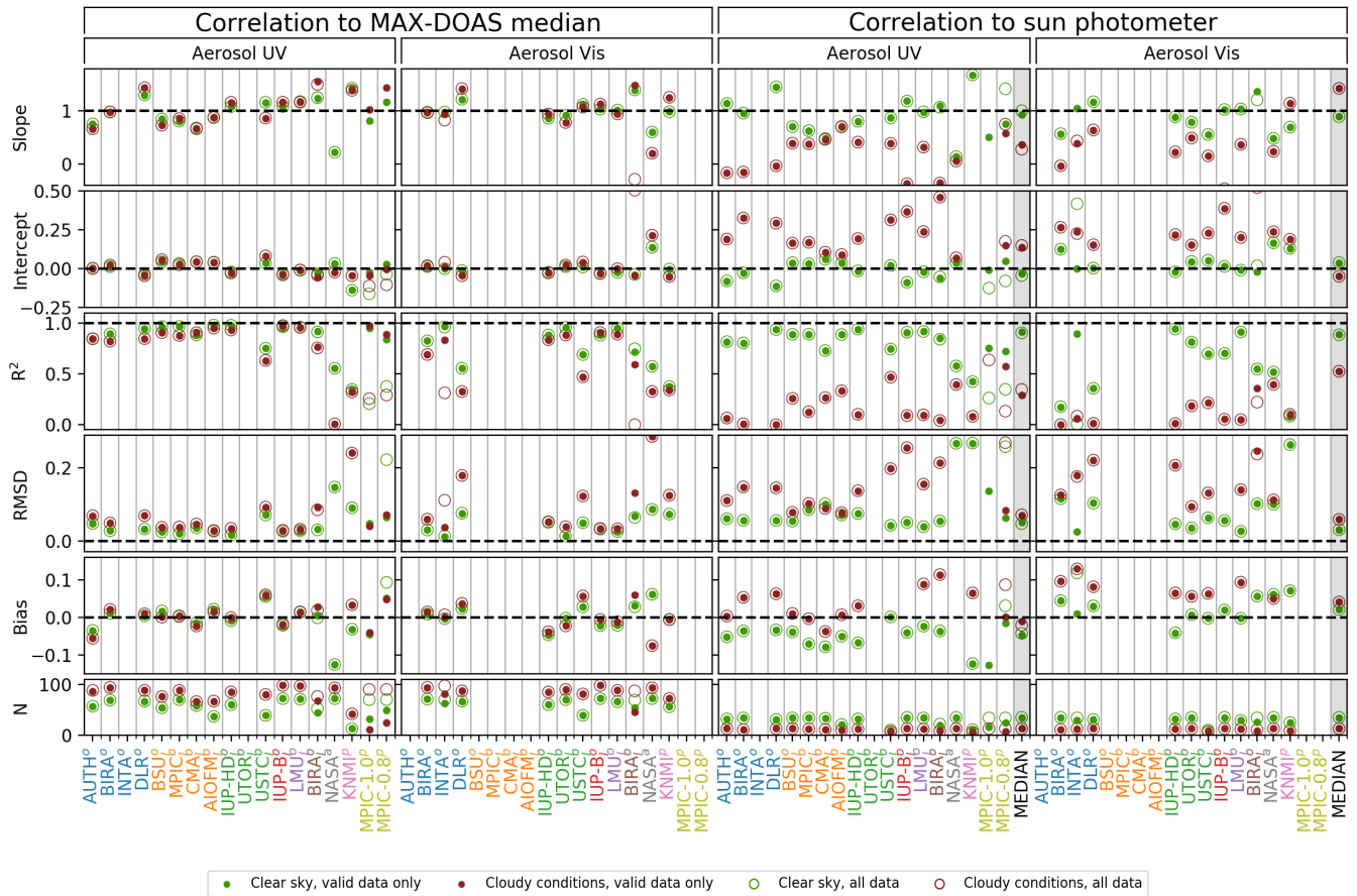
Figure S51. Correlation statistics for AOTs. The two left columns give an impression on the agreement among the institutes, as they show the correlation of the individual participant's retrieved AOT (ordinate of the underlying correlation plot) against the median (abscissa). The two right columns show the correlation against the sun photometer AOT (partial AOT in the case of OEM retrievals) instead of the median. Green and red symbols represent cloud-free and cloudy conditions, respectively. Hollow circles represent values for all submitted data, the dots only consider data points flagged as valid. N is the number of profiles which contributed to the respective data points above. The total number of submitted profiles per participant and species were 170. On the right also the correlation between the MAX-DOAS median results and supporting observations are included (grey shaded columns).
