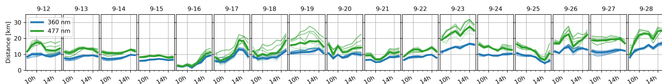
Figure S12. Viewing distance (HSR) of MAX-DOAS instruments during CINDI-2. It was calculated for different elevation angles (1, 2, 3, 4, 5, 6 and 8° with increasing transparency of the curves) and the average value for UV and Vis (thick lines).
