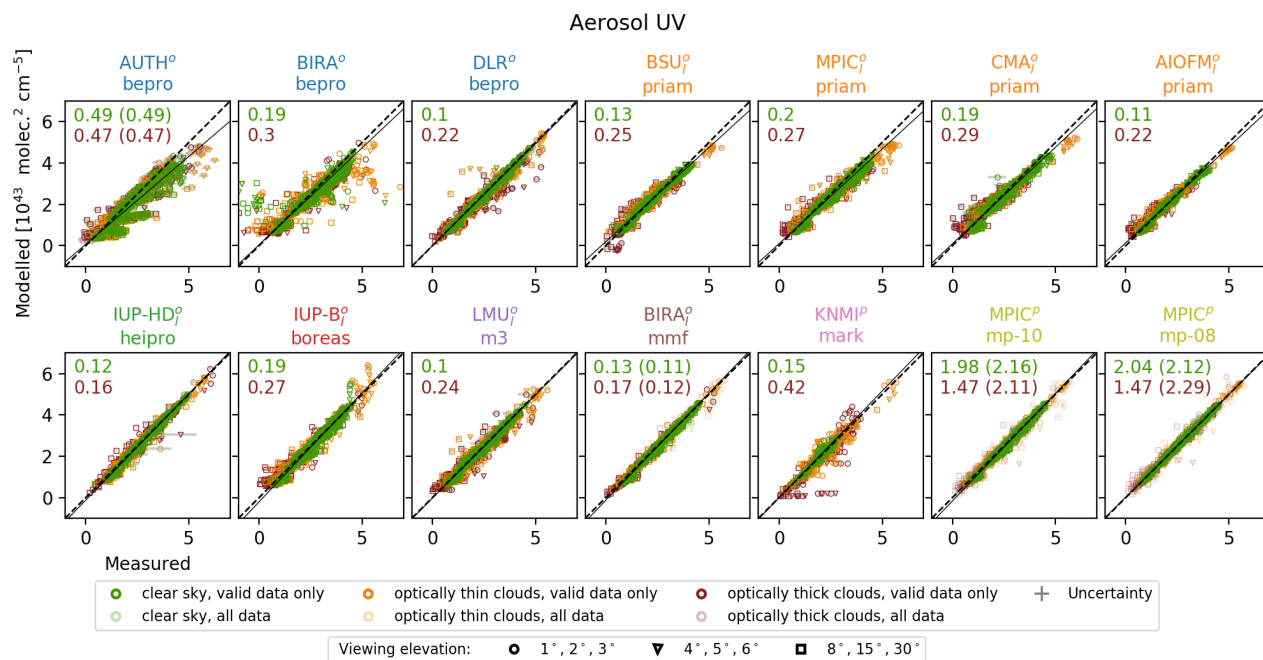
Figure S45. O 4 UV dSCD correlation when profiles are retrieved from the participant's own dSCDs. Marker colours and marker shapes indicate the cloud conditions and viewing elevation angles, respectively. Numbers represent the measurement error weighted RMSD between measured and modelled dSCDs for clear sky (green) and cloudy (red) conditions. Values in brackets were calculated only considering valid data.
