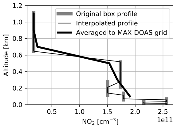
Figure S7. Regridding of an example \text{NO}_2 lidar box profile (27 September 2016, 11:00) to the MAX-DOAS 200 m vertical resolution. In a first step, gaps and overlaps within the box profile are linearly interpolated. The resulting profile is then averaged within the MAX-DOAS retrieval layers.
