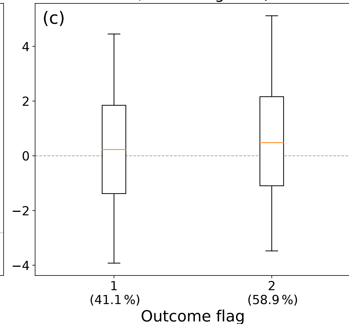
WarnLevel < 3 ; CloudFlag = 3 (N = 383 591)
