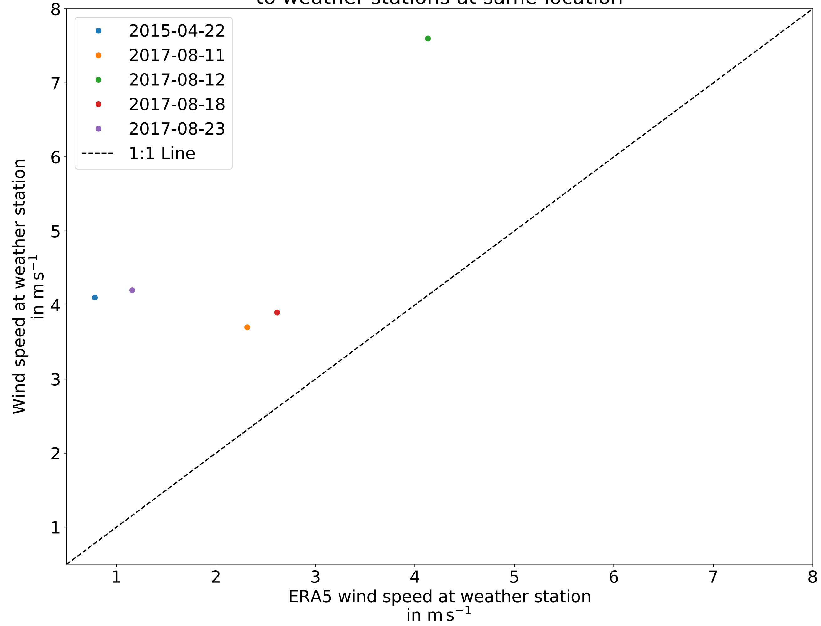
Comparison ERA5 wind speed lowest 50 m to weather stations at same location
