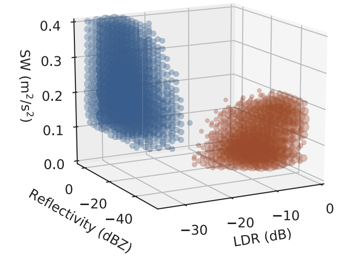
(d2) LT 00:00-06:00, height 1.8-2.7 km
