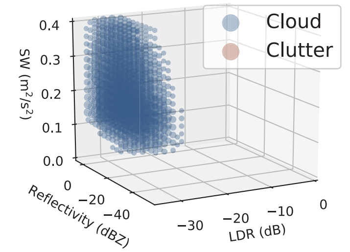
(d1) LT 00:00-06:00, height 2.7-3.6 km
