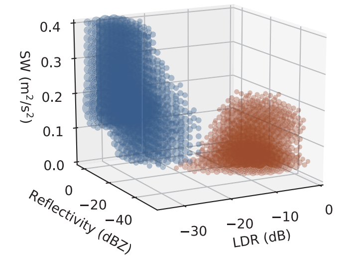
(d3) LT 00:00-06:00, height below 1.8 km
