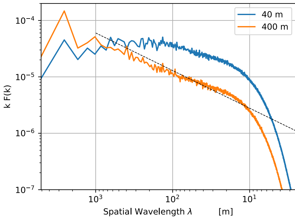
(c) Specific humidity q
