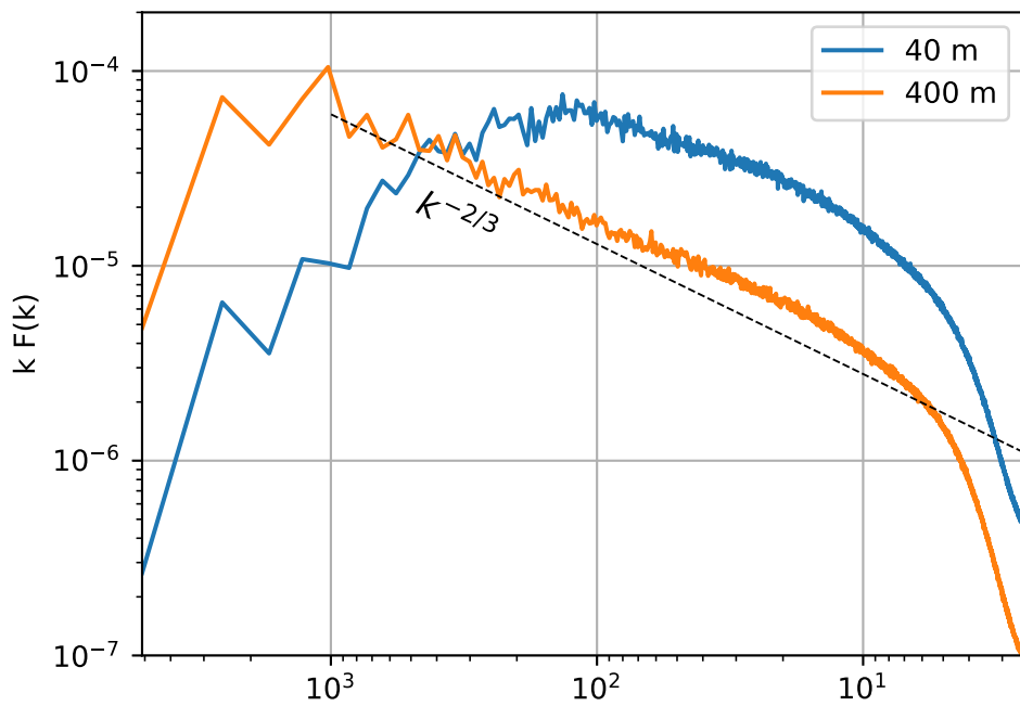
(c) Specific humidity q
