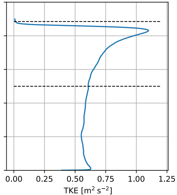
(c) Turbulent Kinetic Energy
