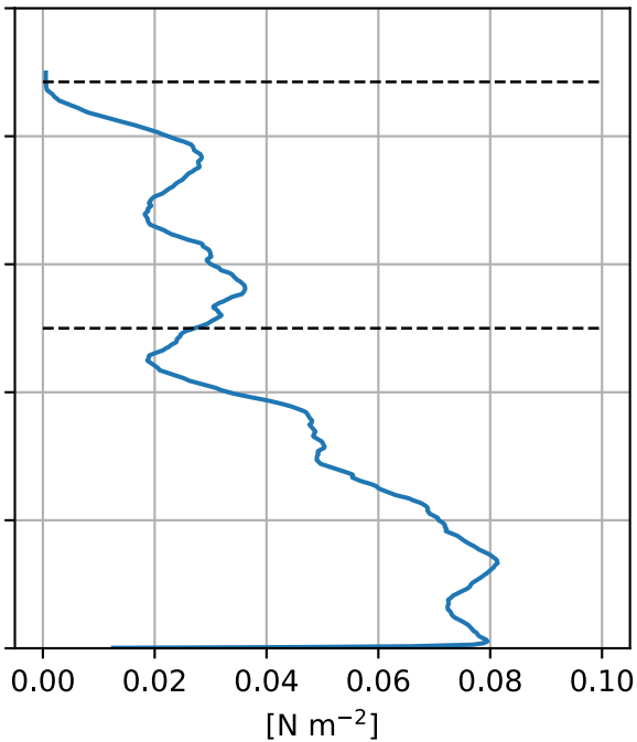
(b) Momentum Flux
