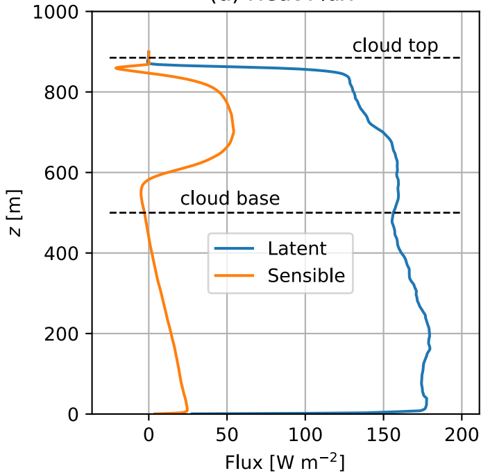
(a) Heat Flux
