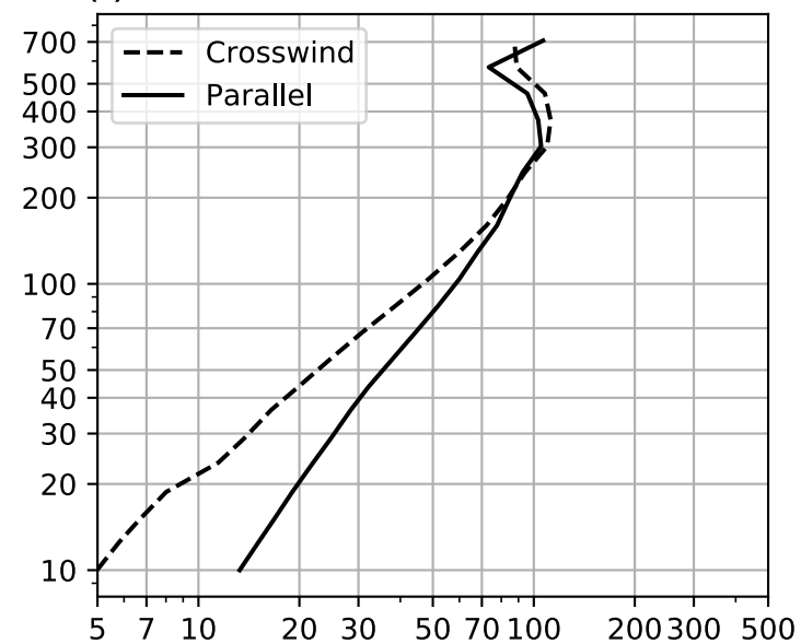
(f) Sensible Heat Flux
