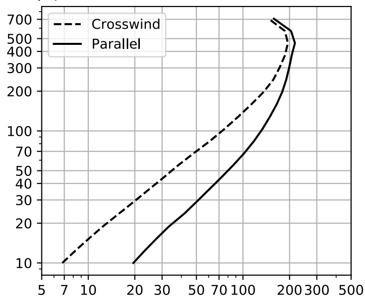
(e) Vertical Wind w
