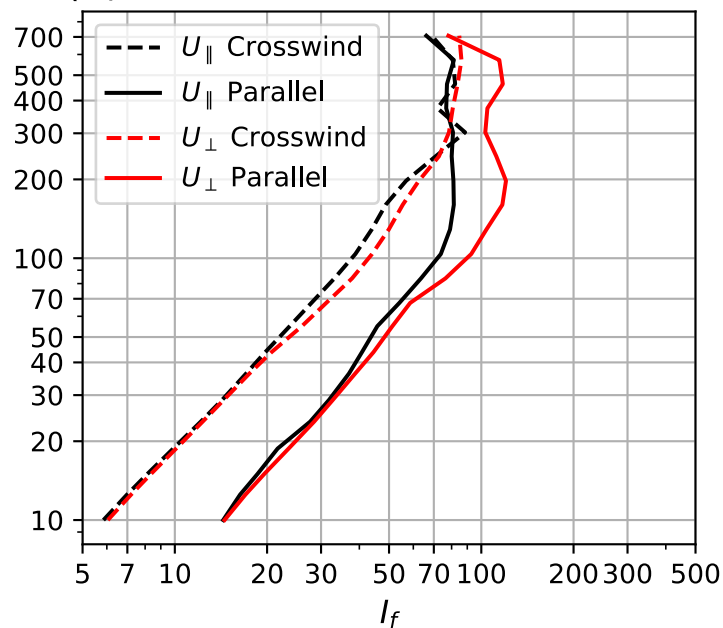
(h) Momentum Flux
