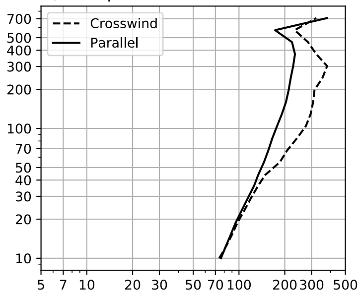
(b) Temperature T
