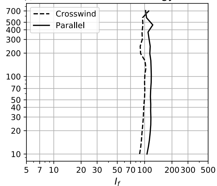
(i) Turbulent Kinetic Energy
