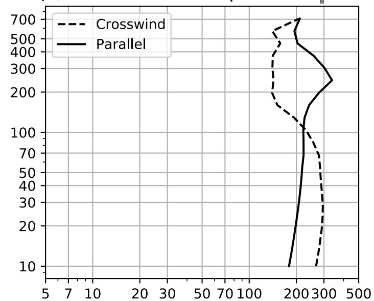
(c) Horiz. Wind Component U_{\parallel}
