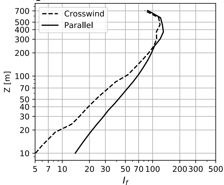
(g) Latent Heat Flux
