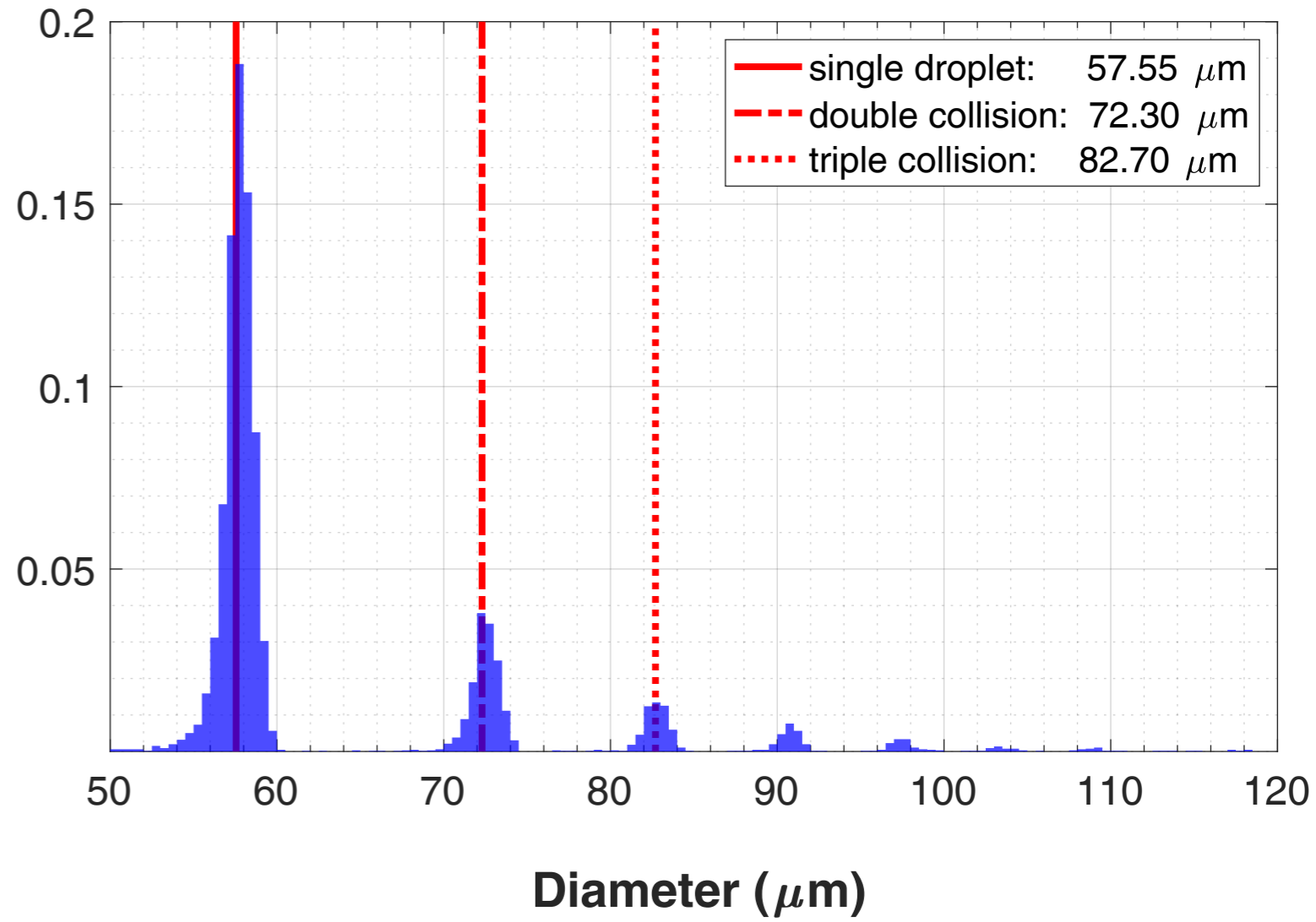
(b) FMAG: d=57.55 \mu\text{m}
