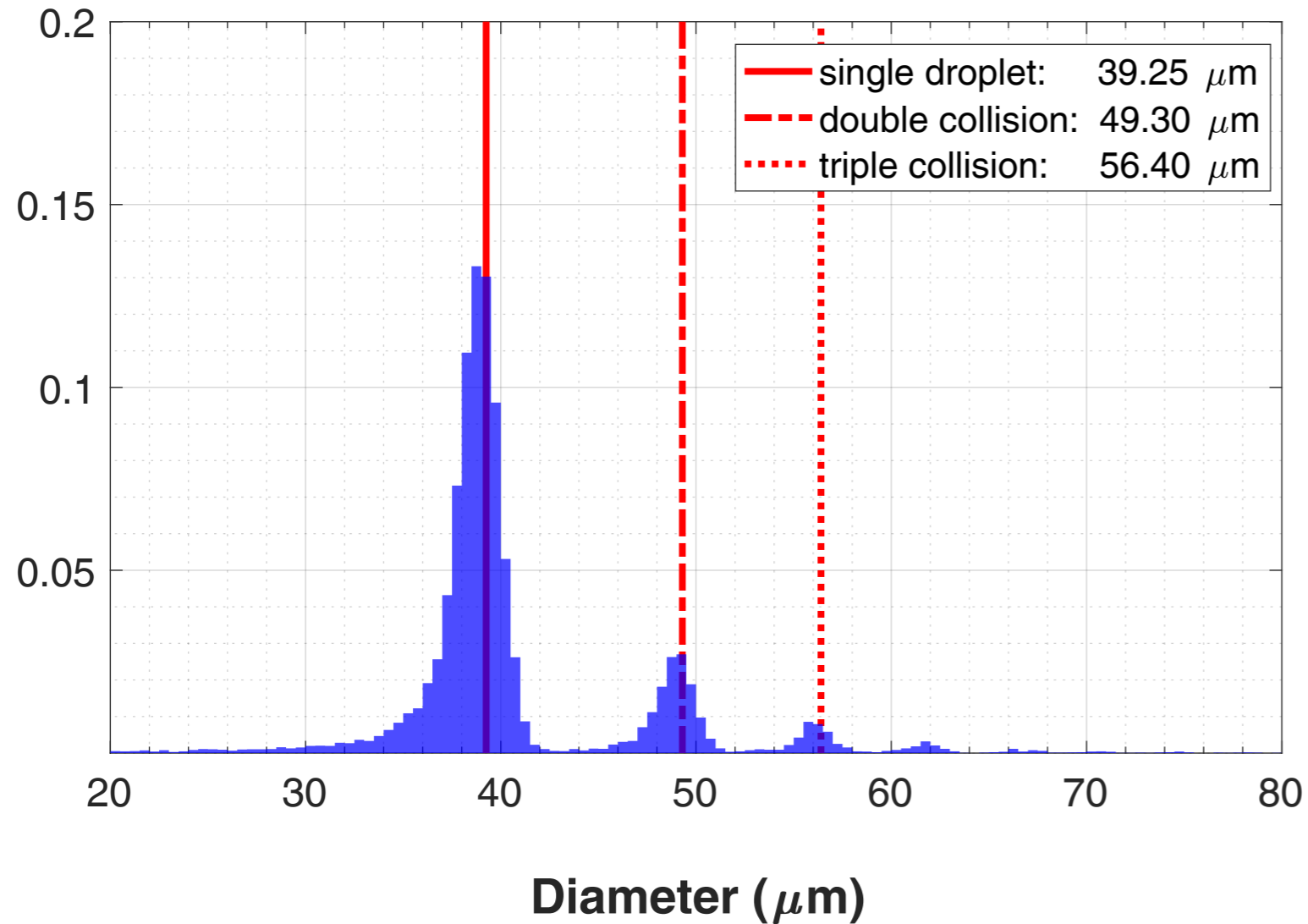
(a) FMAG: d=39.25 \mu\text{m}
