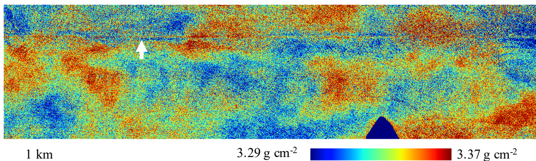
Column average H 2 O vapor, flight line B (ang20180512t053942)
