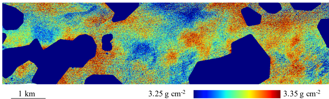
Column average H 2 O vapor, flight line A (ang20180514t060206)
