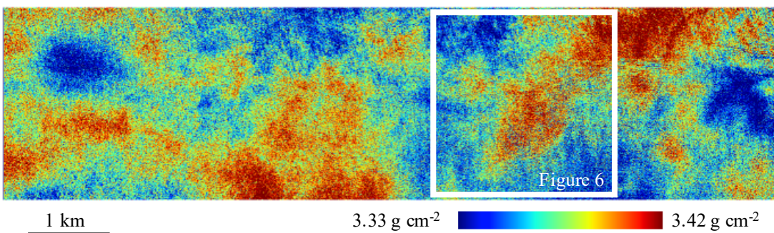
Column average H 2 O vapor, flight line C (ang20180514t055115)
