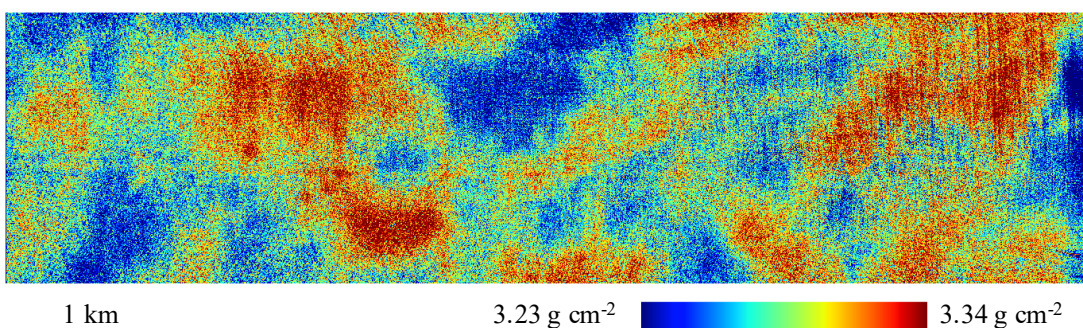
Column average H 2 O vapor, flight line D (ang20180514t060206)
