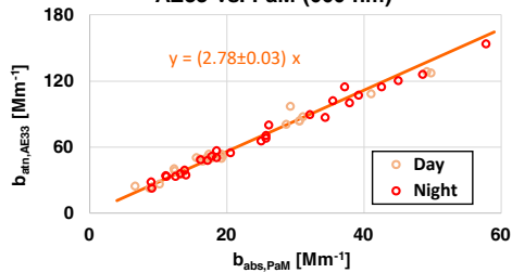
AE33 vs. PaM (880 nm)
