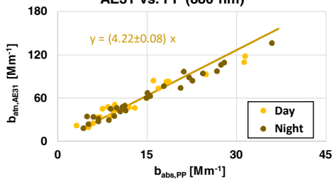
AE31 vs. PP (880 nm)
