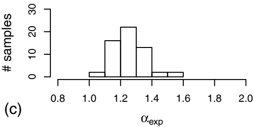
AE33_4 \lambda _C PP
