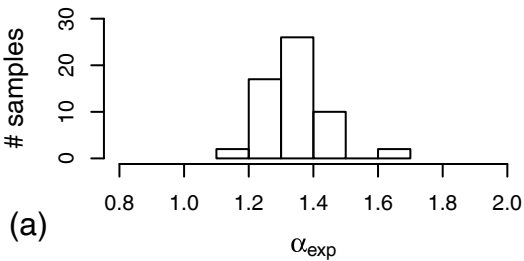
AE33_4 \lambda _C 0
