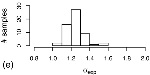
AE33_4 \lambda _C PaM
