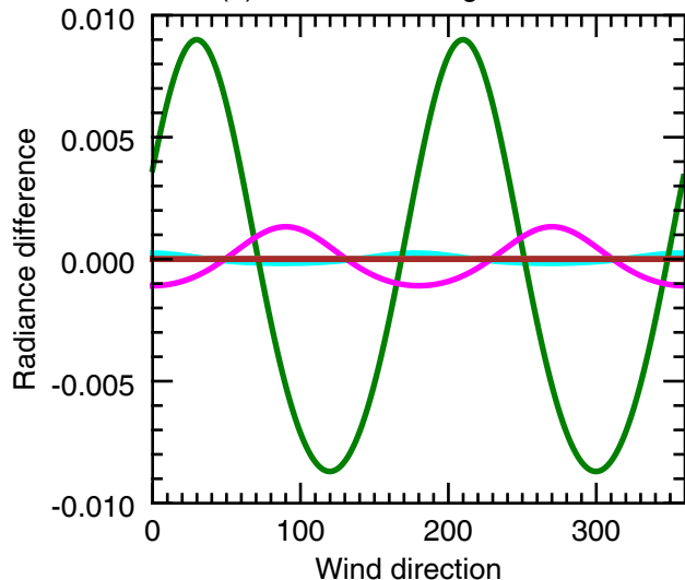
(b) Vector - scalar glint radiance
