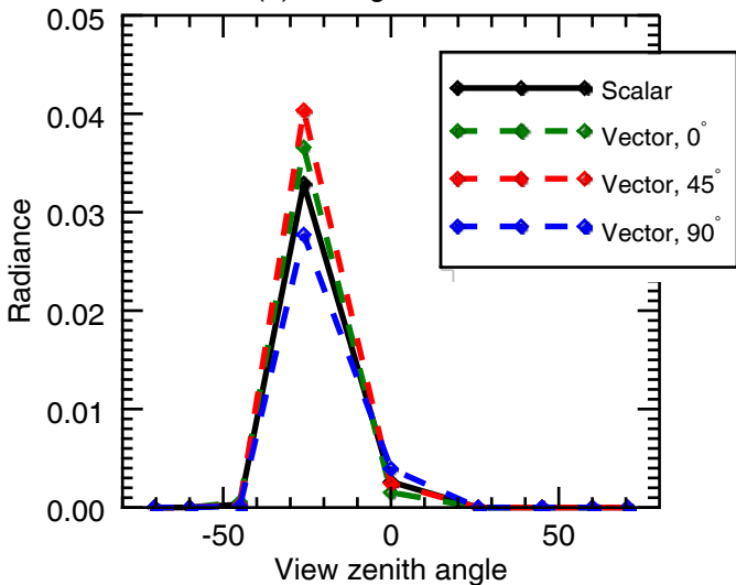
(a) TOA glint radiance
