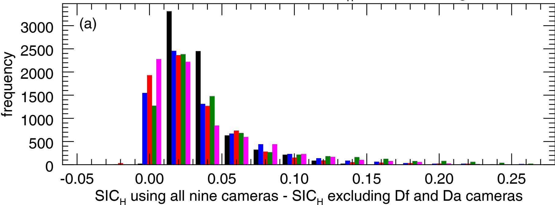
Nine vs. seven MISR camera SIC_H difference histogram
