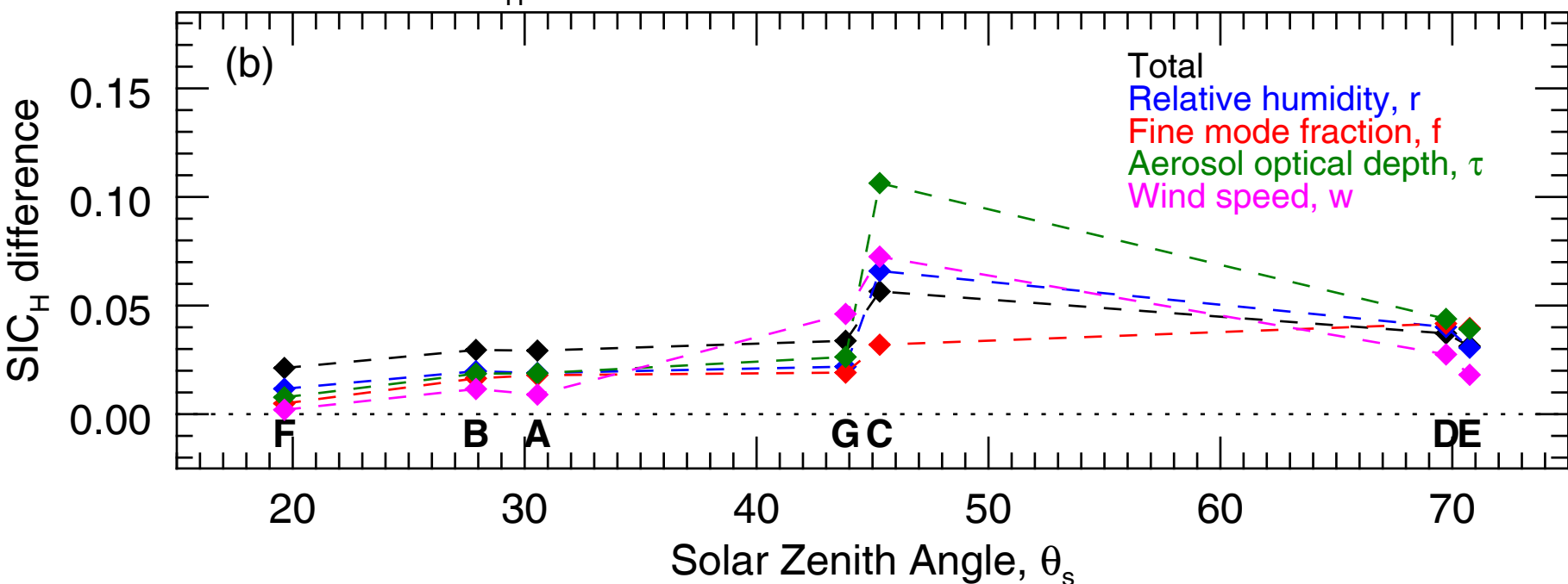
SIC_H median difference between 9 and 7 views
