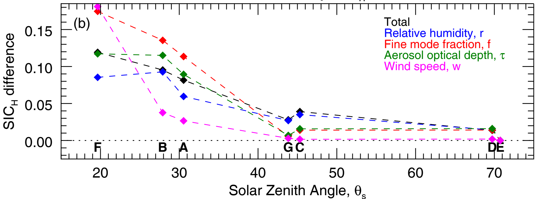
Scalar vs. Vector wind uncertainty, SIC_H median difference
