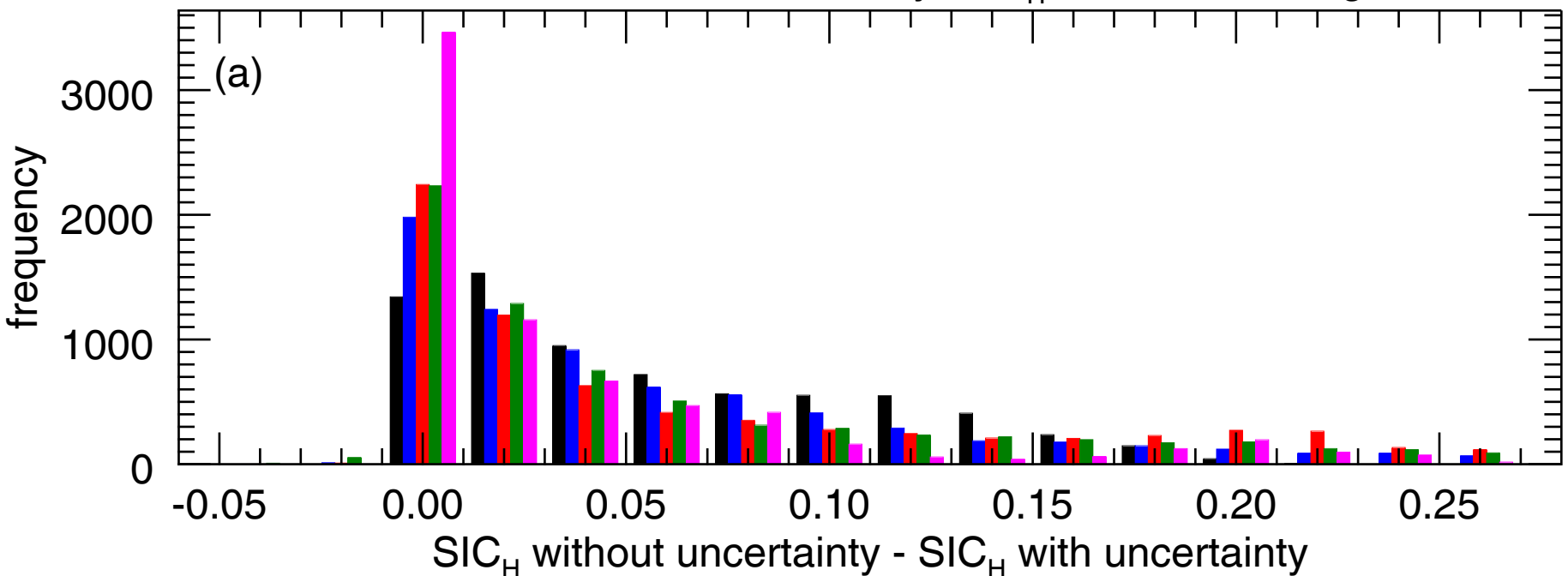
Scalar vs. Vector wind uncertainty, SIC_H difference histogram
