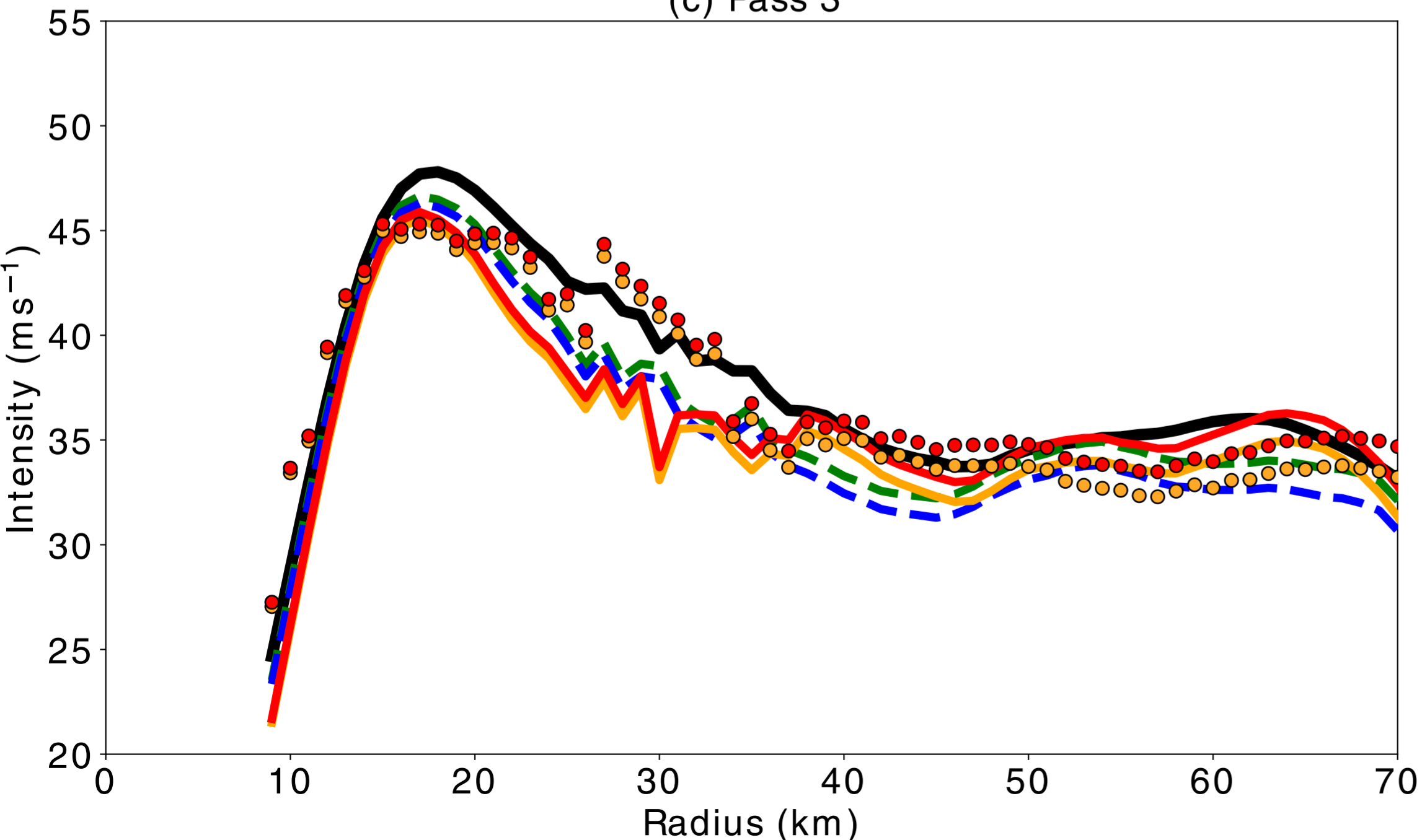
(c) Pass 3
