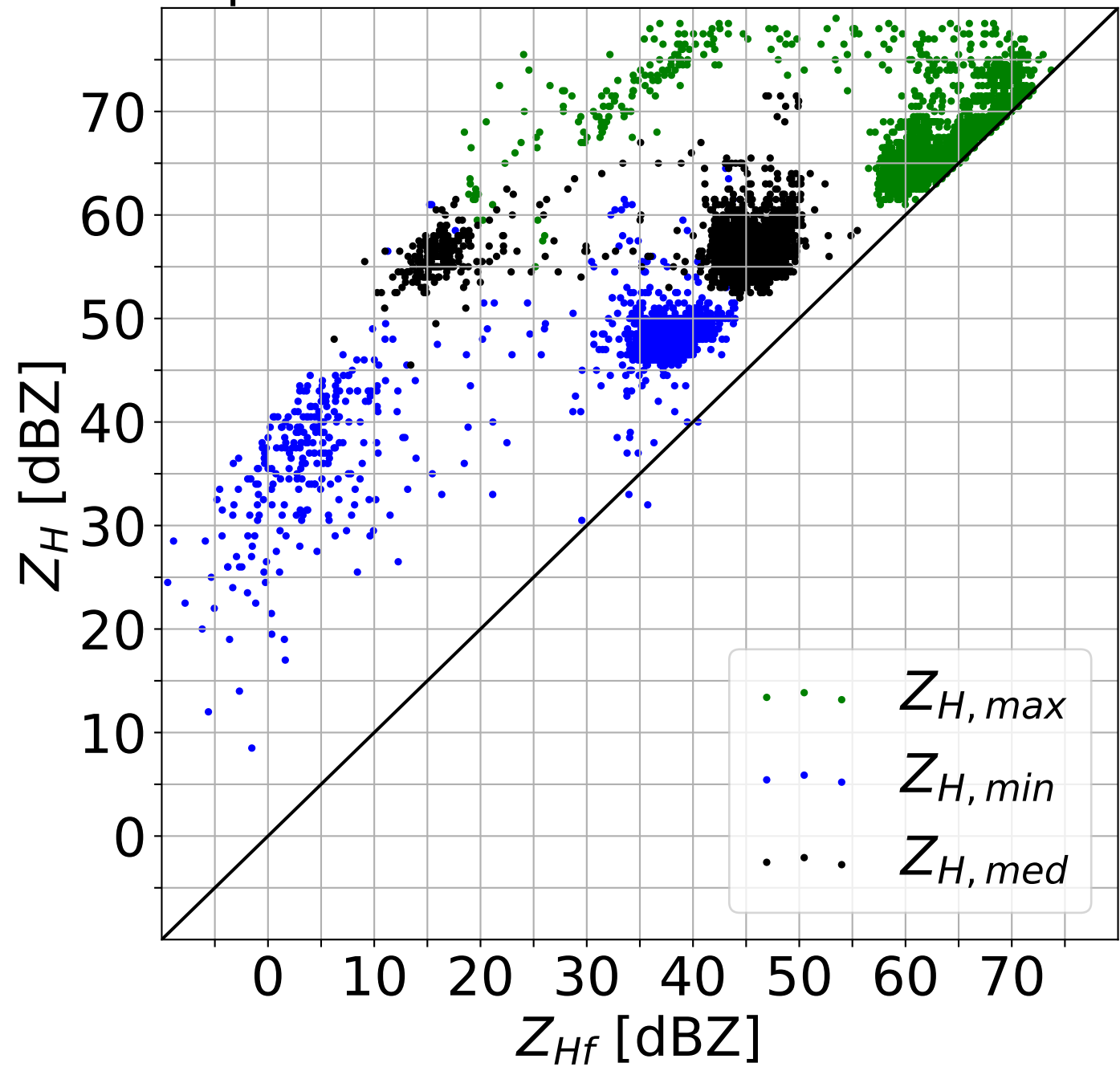
Scatter plot between filtered and unfiltered Z_H
