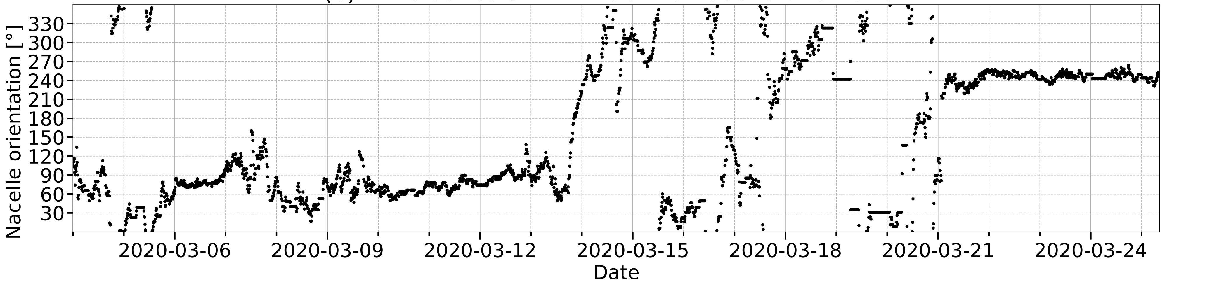
(b) Time series of WT1 relative nacelle orientation
