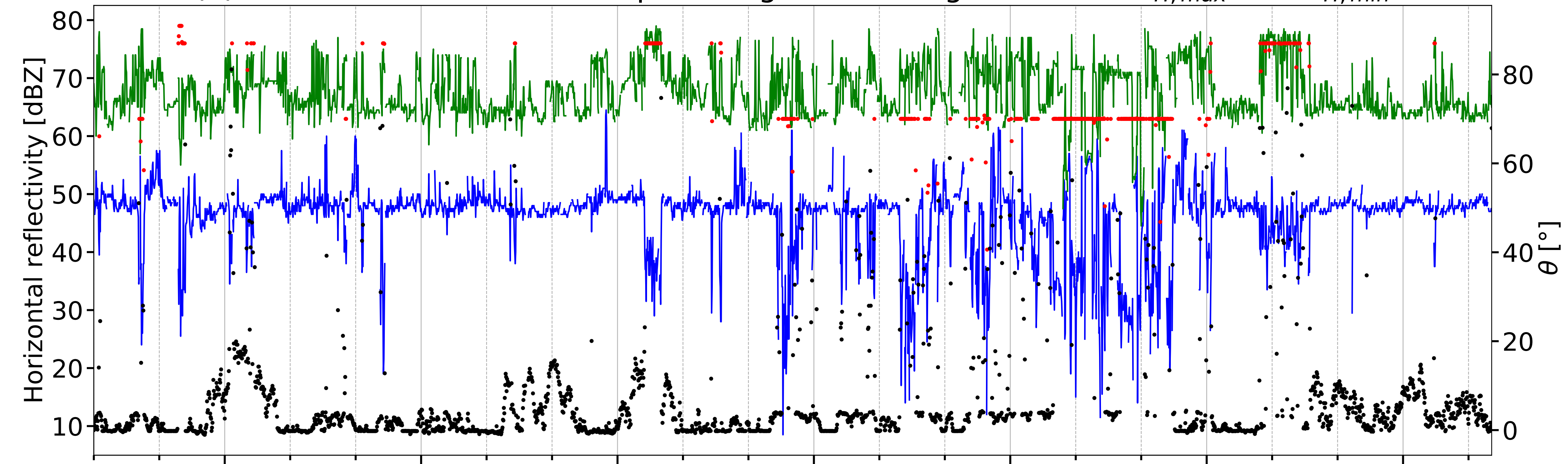
(a) Time series of WT1 blade pitch angle \theta , moving median of Z_{H,max} and Z_{H,min}
