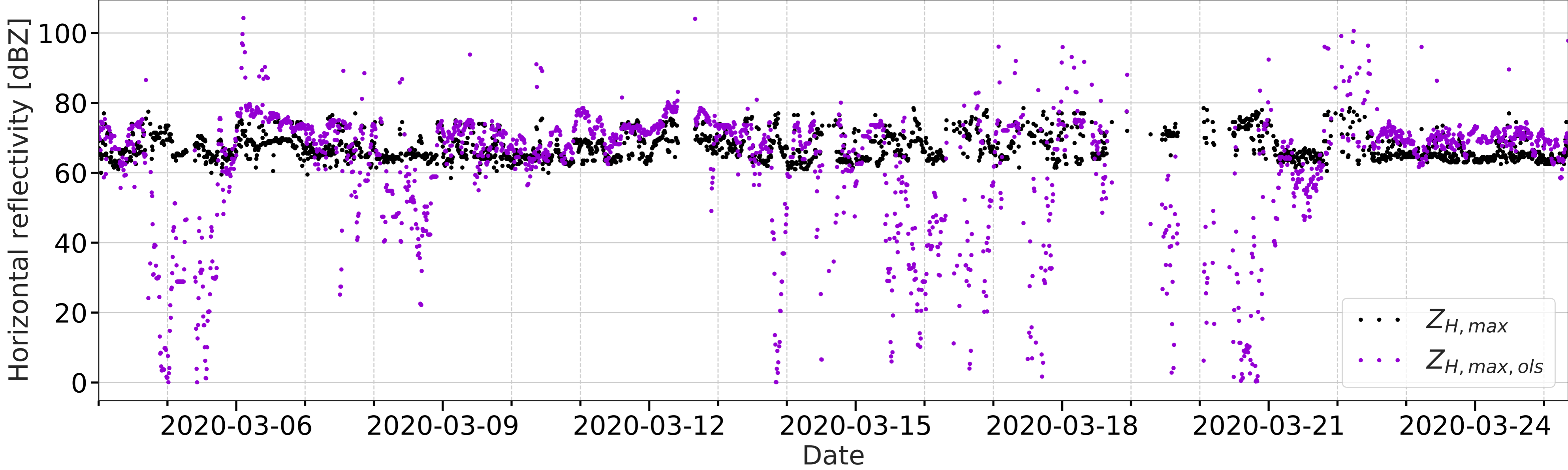
Time series comparison between moving Z_{H,max} and rebuilt Z_{H,max,ols} when r_s \geq 1 rpm
