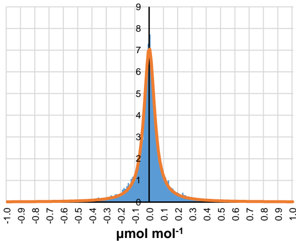
(a) no. of intakes: 3; sampling period: 120 s; \gamma = 0.045
