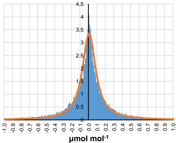
(b) no. of intakes: 3; sampling period: 400 s; \gamma = 0.095
