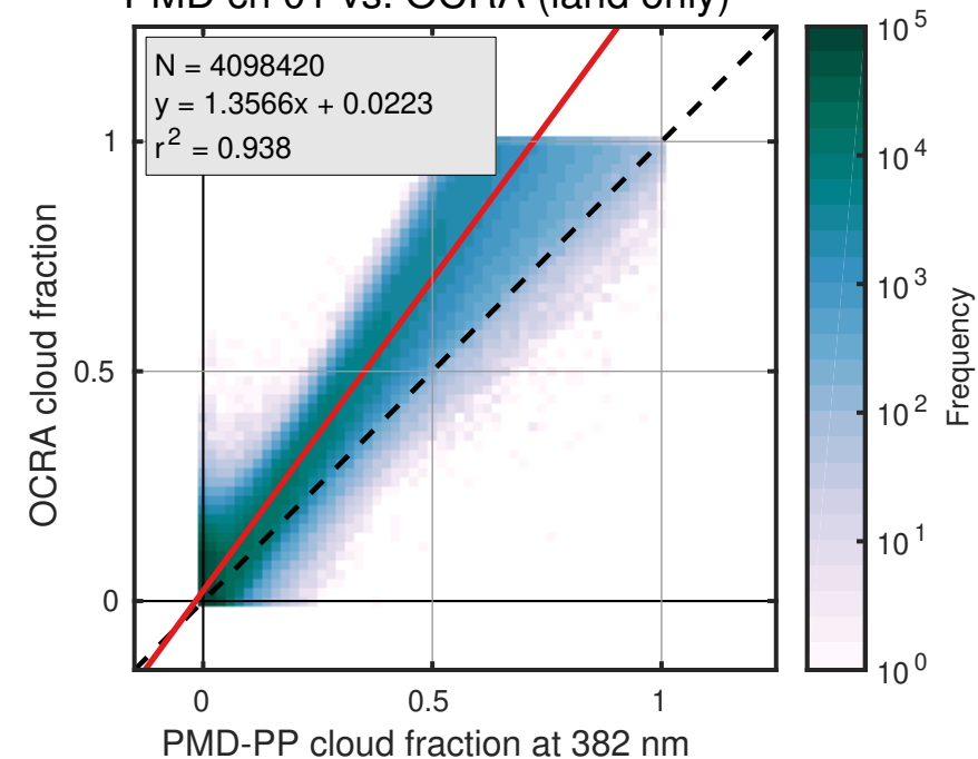
(a) PMD ch 01 vs. OCRA (land only)
