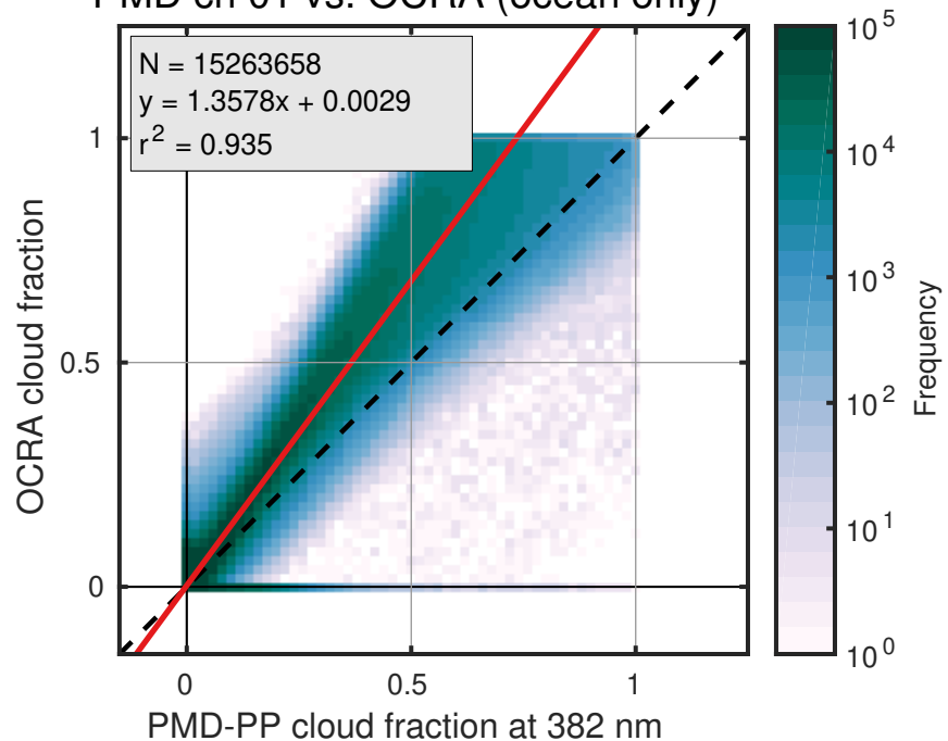
(b) PMD ch 01 vs. OCRA (ocean only)
