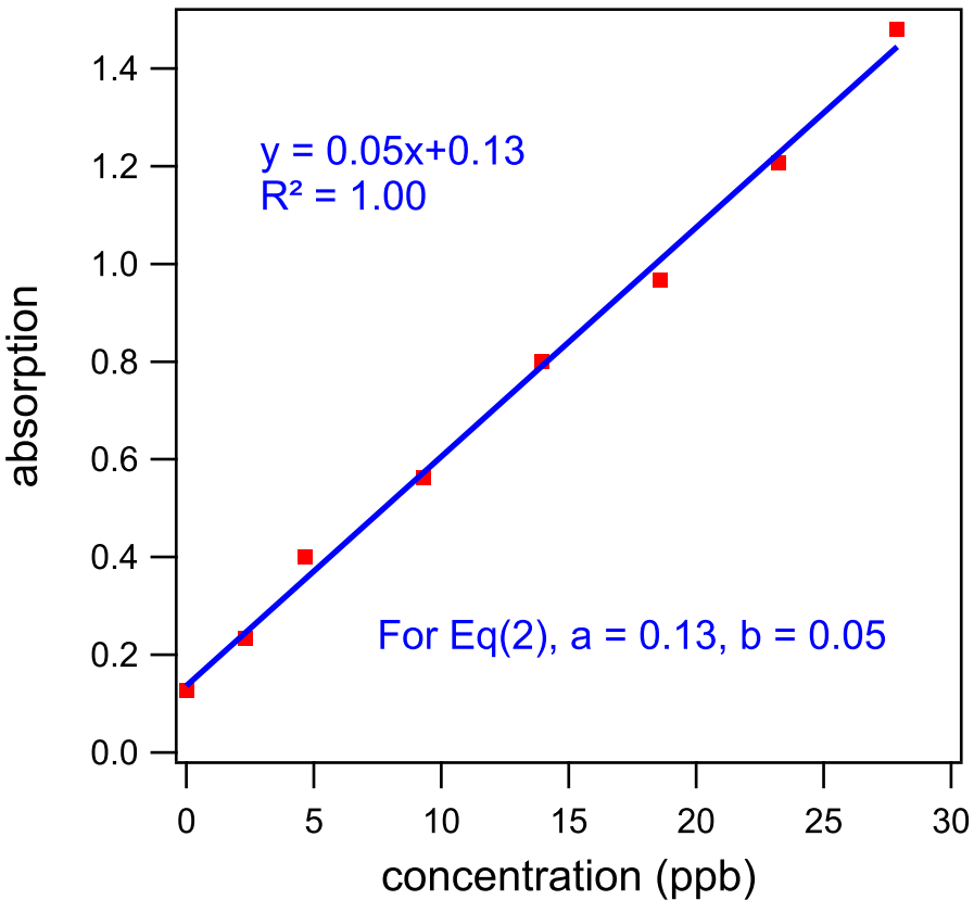
(a) Calibration curve of Fe
