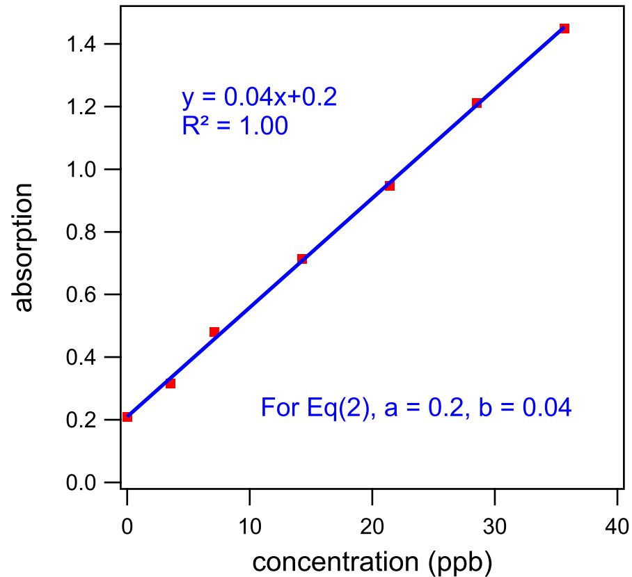
(b) Calibration curve of Cu
