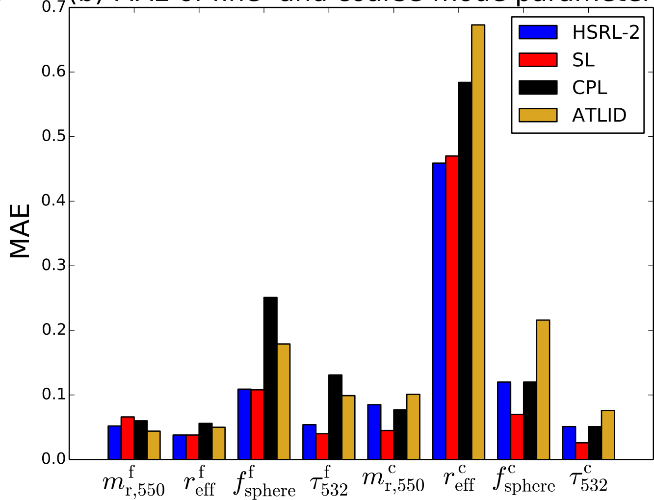
(b) MAE of fine- and coarse-mode parameters
