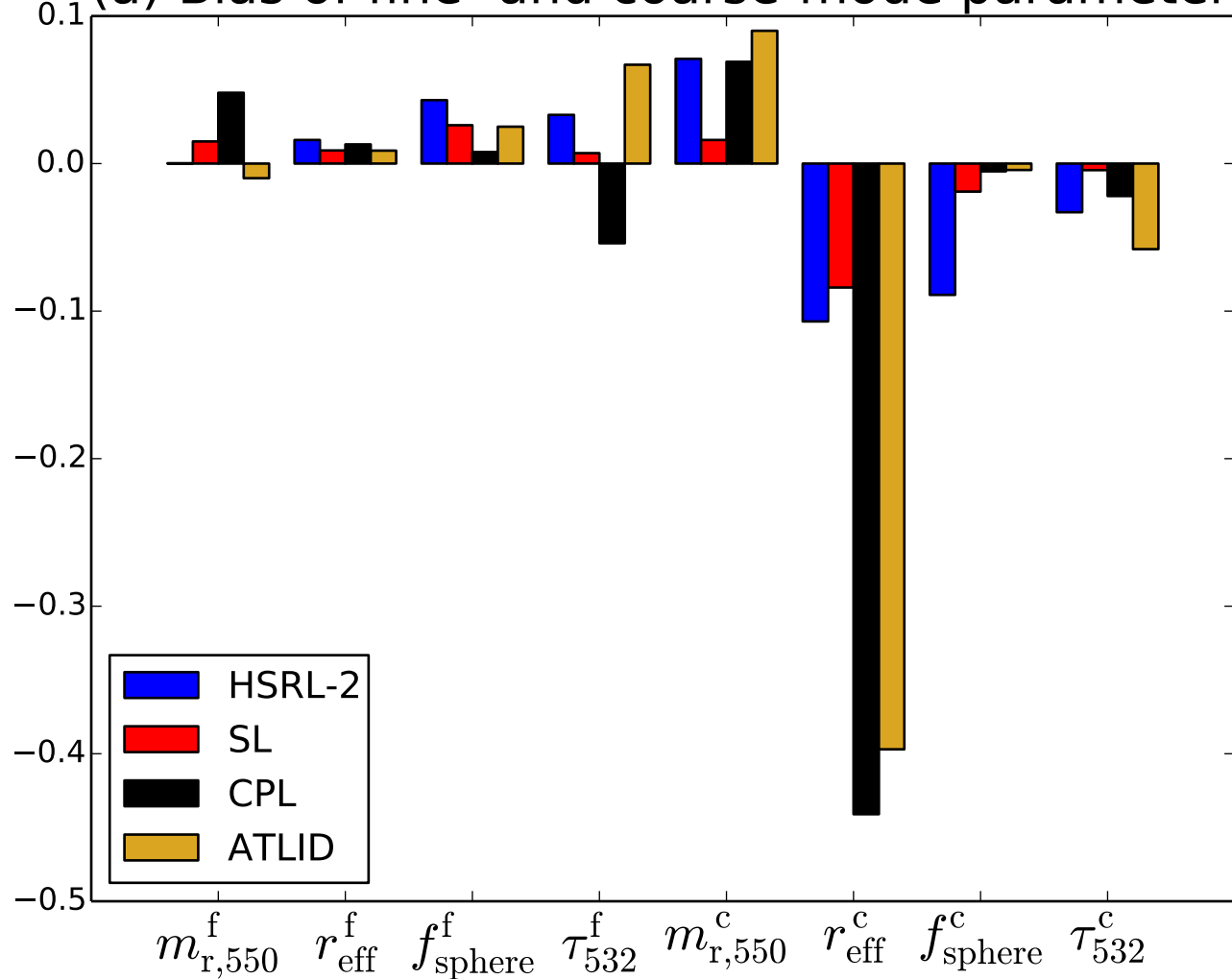
(a) Bias of fine- and coarse-mode parameters
