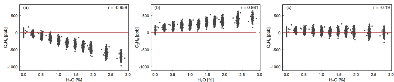
Figure 3. \text{H}_2\text{O} influence on corrected \text{C}_2\text{H}_6 . Water vapor is increased in small steps for 4 h while measuring Target Gas 1. The three panels show the result of applying different water correction protocols for the next steps: (a) no correction, (b) high-humidity interference correction, (c) low-humidity interference correction. In all cases, for \text{H}_2\text{O} = 0.00\% , \text{C}_2\text{H}_6 is corrected using low-humidity interference correction. The red line represents 0 ppb.
