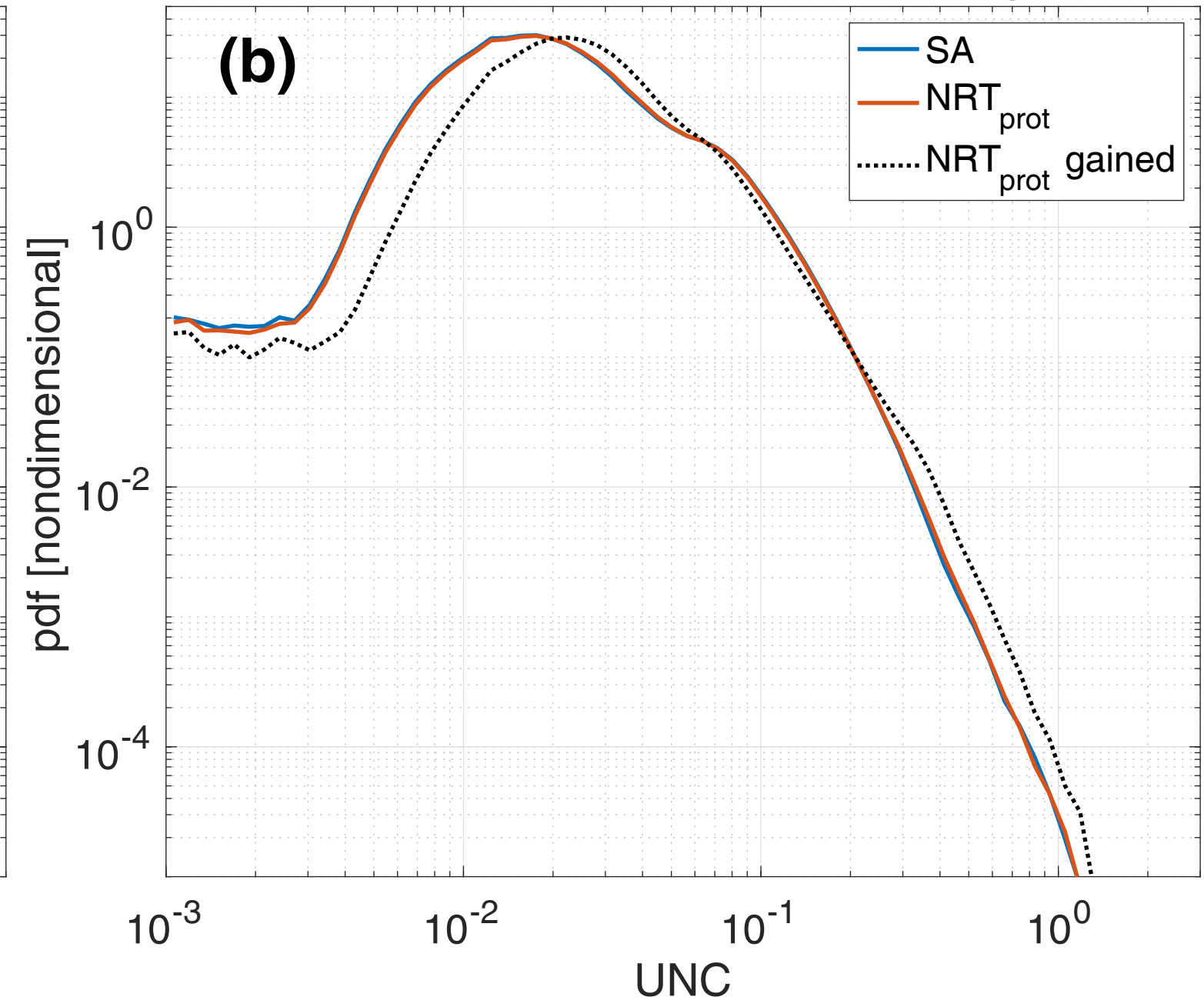
UNC retrievals (March+April+May)
