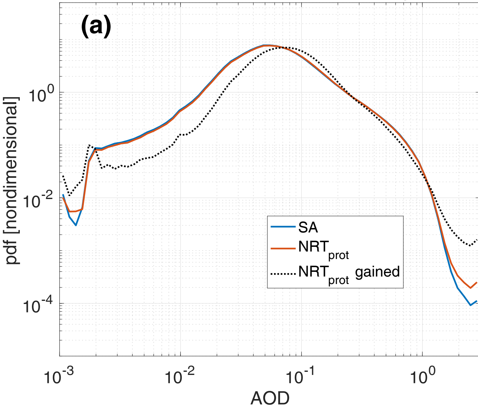
AOD retrievals (March+April+May)
