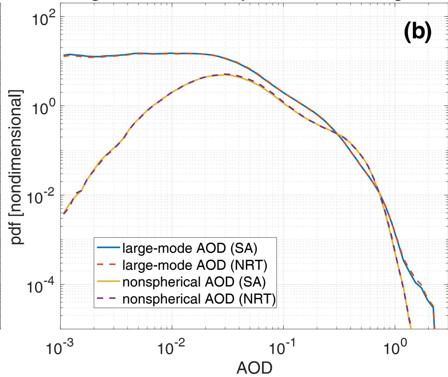
Large-mode and nonspherical AOD histograms
