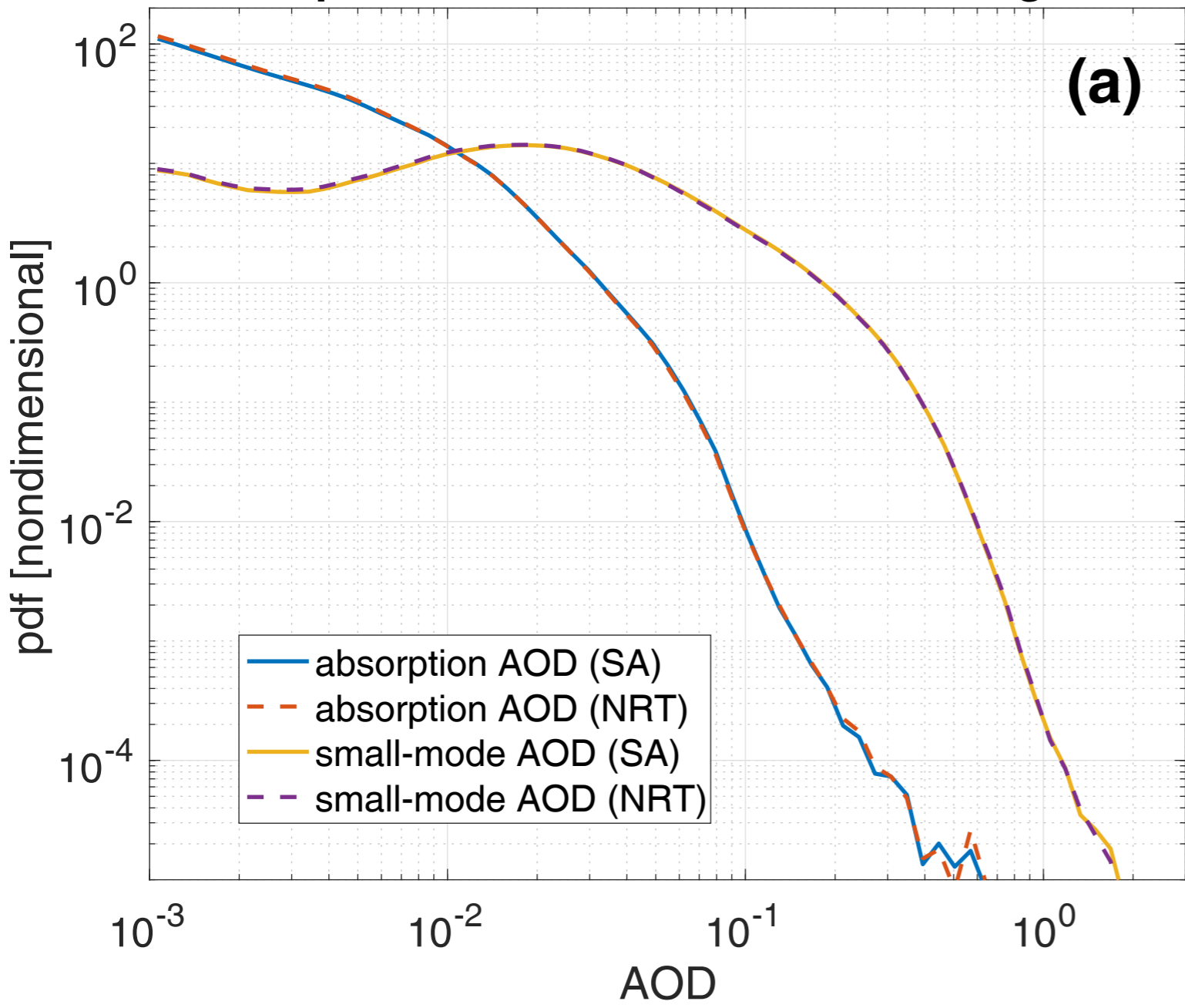
Absorption and small-mode AOD histograms
